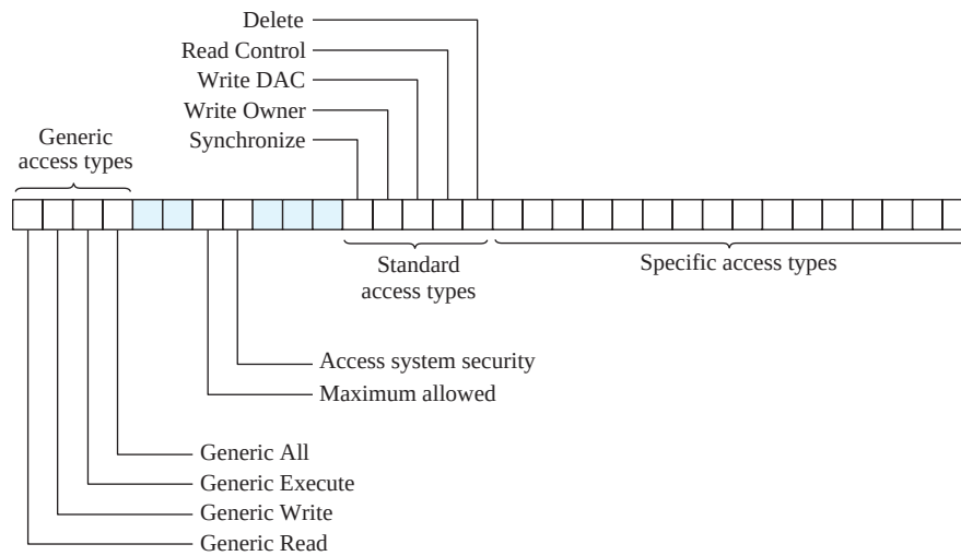
Figure 15.12 Access Mask
