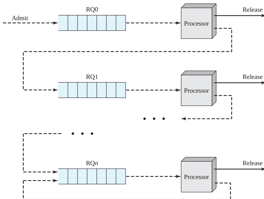
Figure 9.10 Feedback Scheduling
