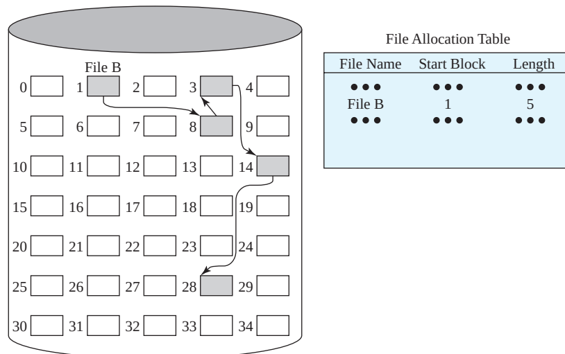
Figure 12.9 Chained Allocation
