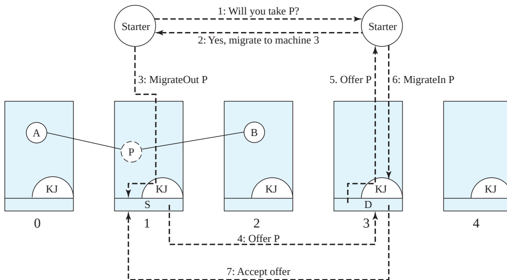
Figure 18.2 Negotiation of Process Migration
