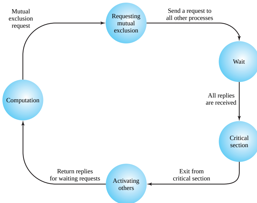
Figure 18.10 State Diagram for Algorithm in
