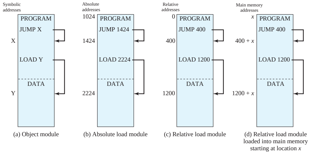
Figure 7.17 Absolute and Relocatable Load Modules
