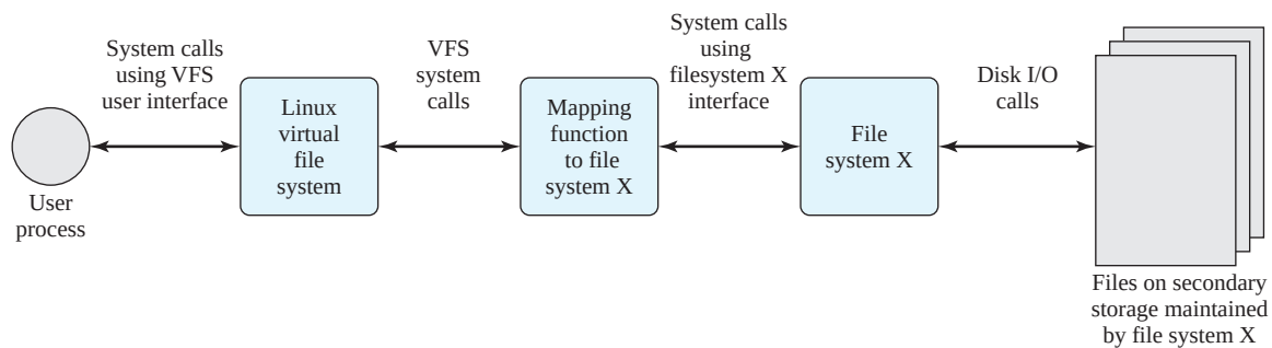
Figure 12.18 Linux Virtual File System Concept
