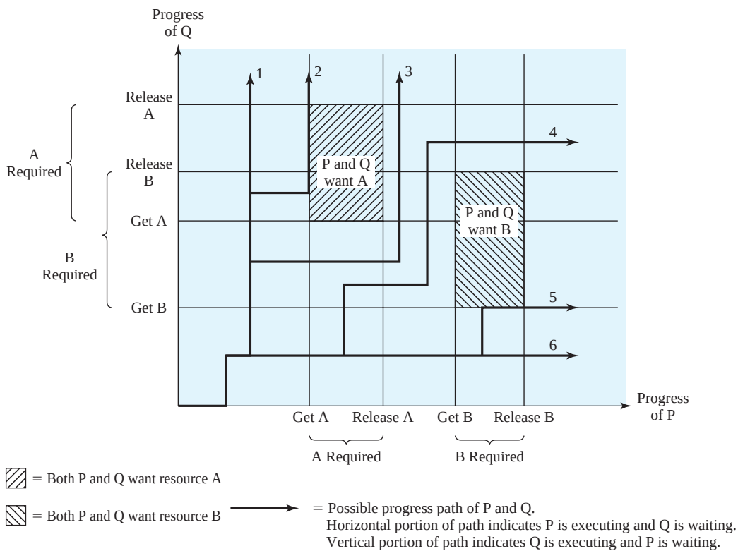
Figure 6.3 Example of No Deadlock [BAC003]
