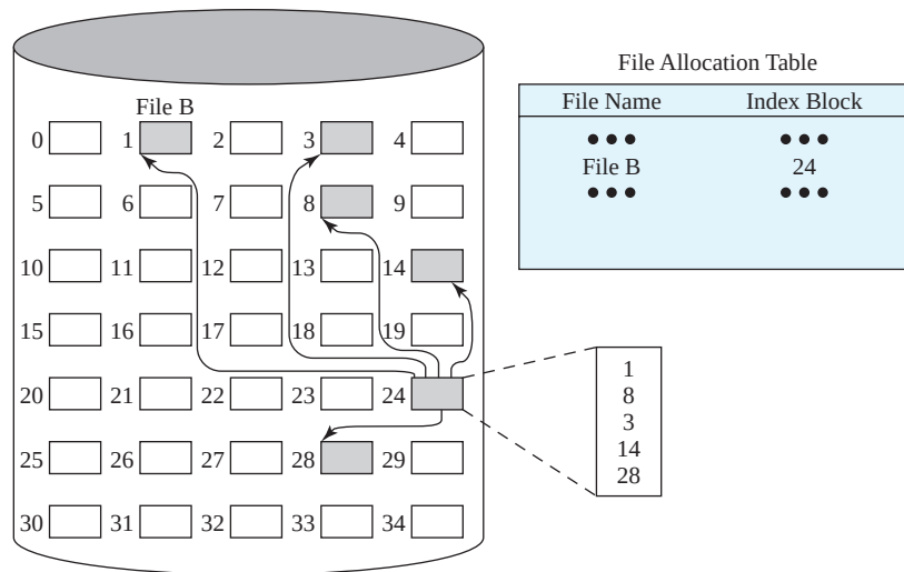
Figure 12.11 Indexed Allocation with Block Portions
