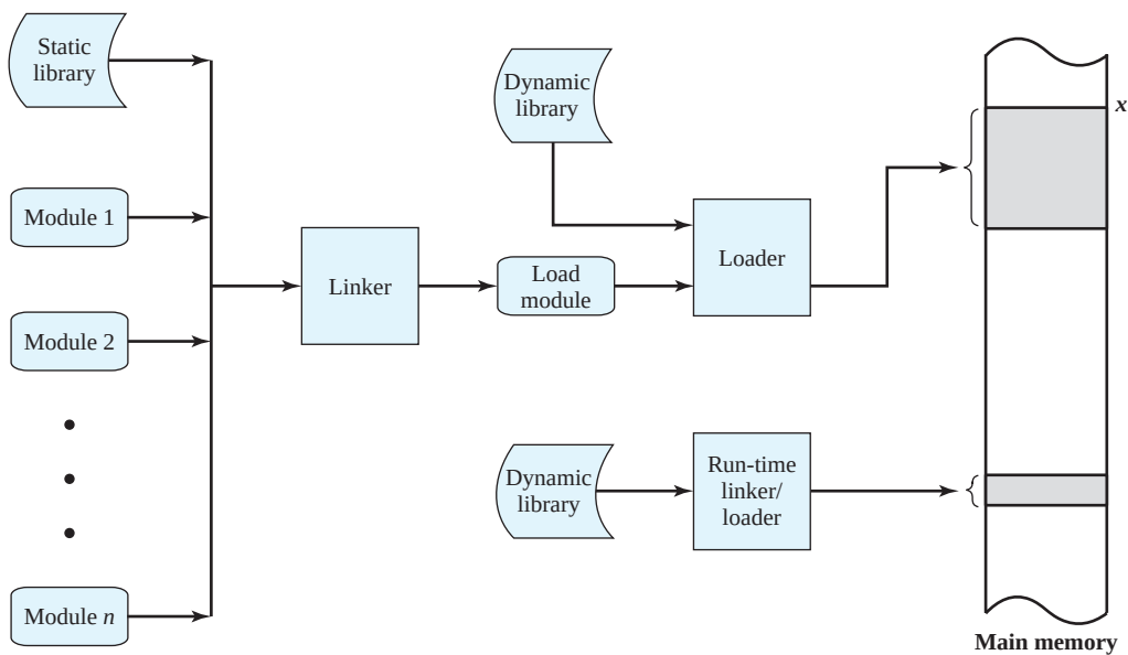
Figure 7.16 A Linking and Loading Scenario
