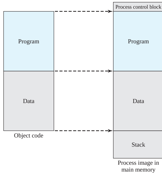
Figure 7.15 The Loading Function
