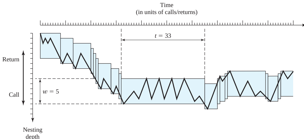
Figure 1.20 Example Call-Return Behavior of a Program
