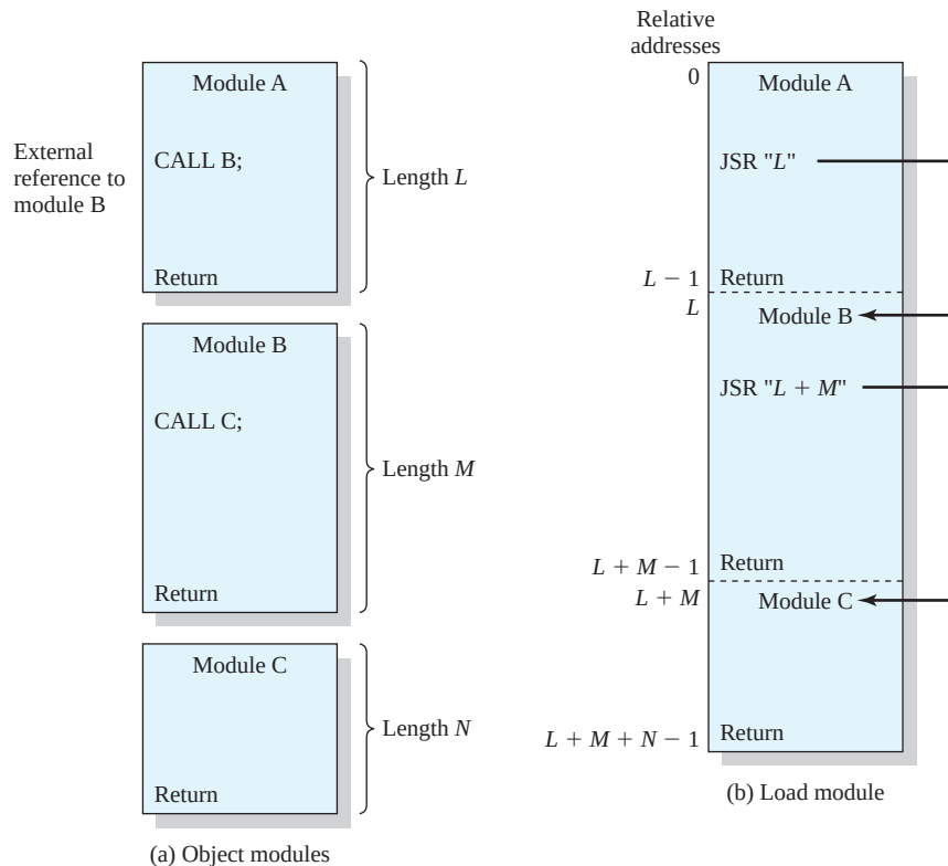
Figure 7.18 The Linking Function
