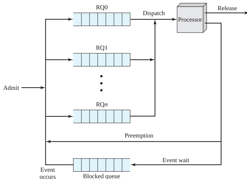
Figure 9.4 Priority Queuing
