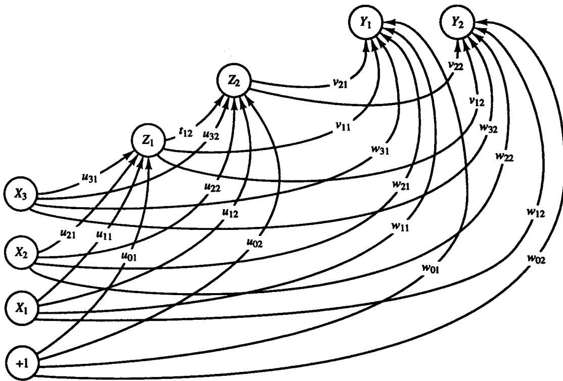
Figure 7.29 Cascade correlation network.
