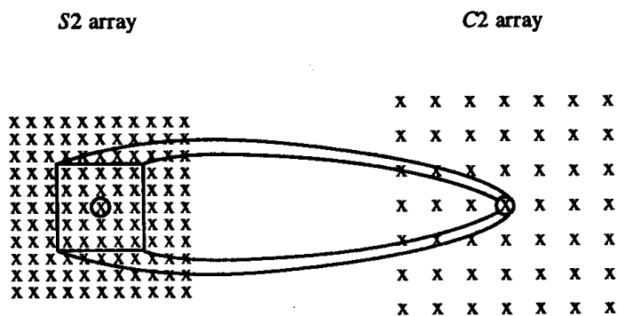
Figure 7.35 Connections from S2 array to C2 array.
