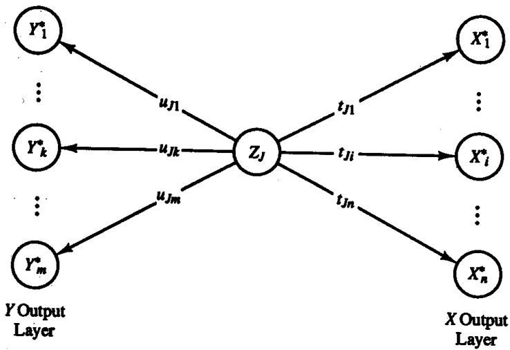
Figure 4.43 Second phase of counterpropagation training.
