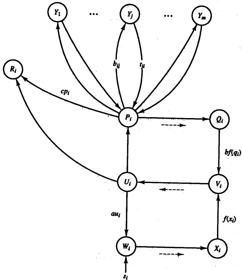
Figure 5.4 Typical ART2 architecture [Carpenter & Grossberg, 1987b].
