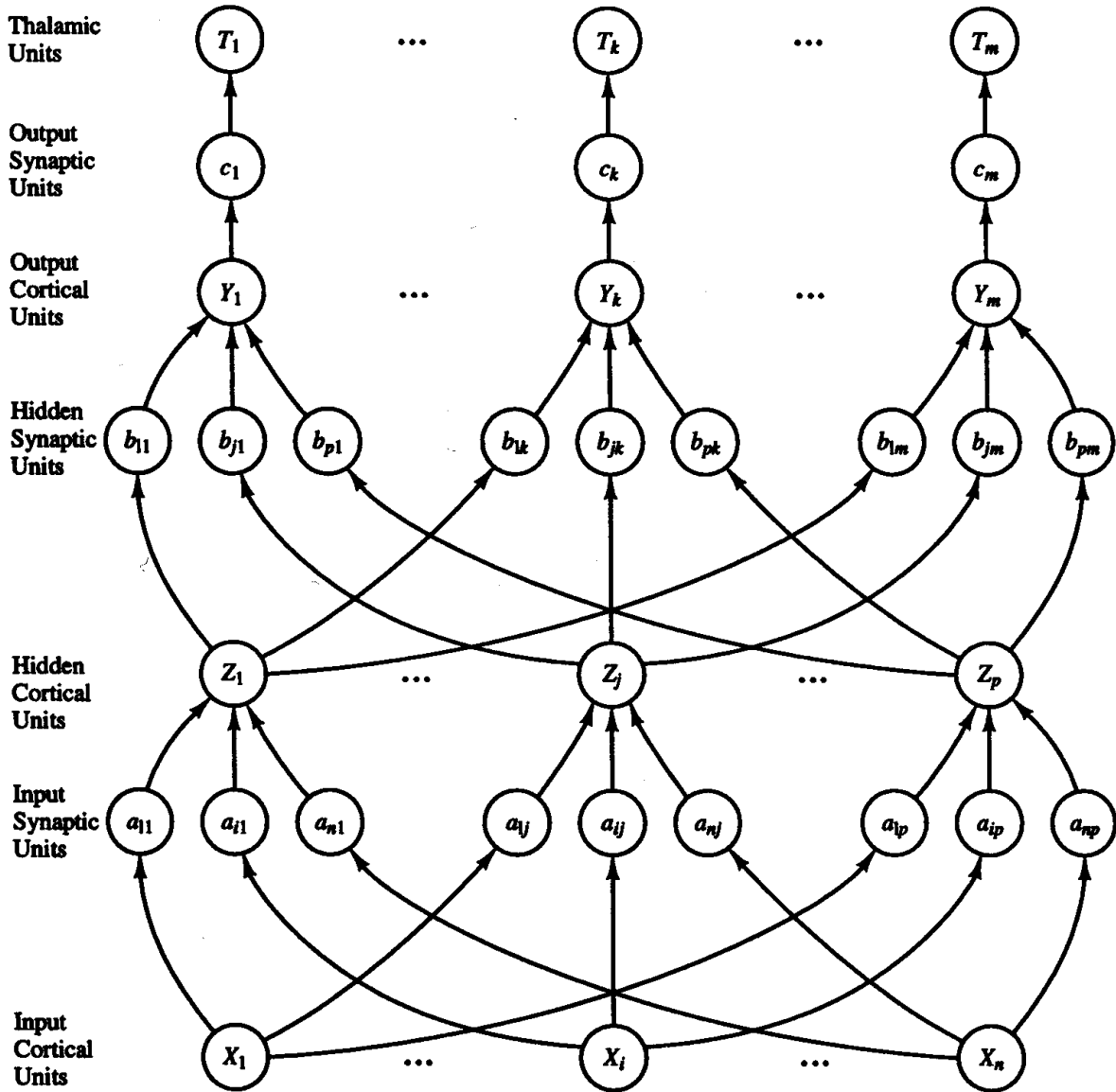
Figure 6.10 Strictly local backpropagation neural net.
