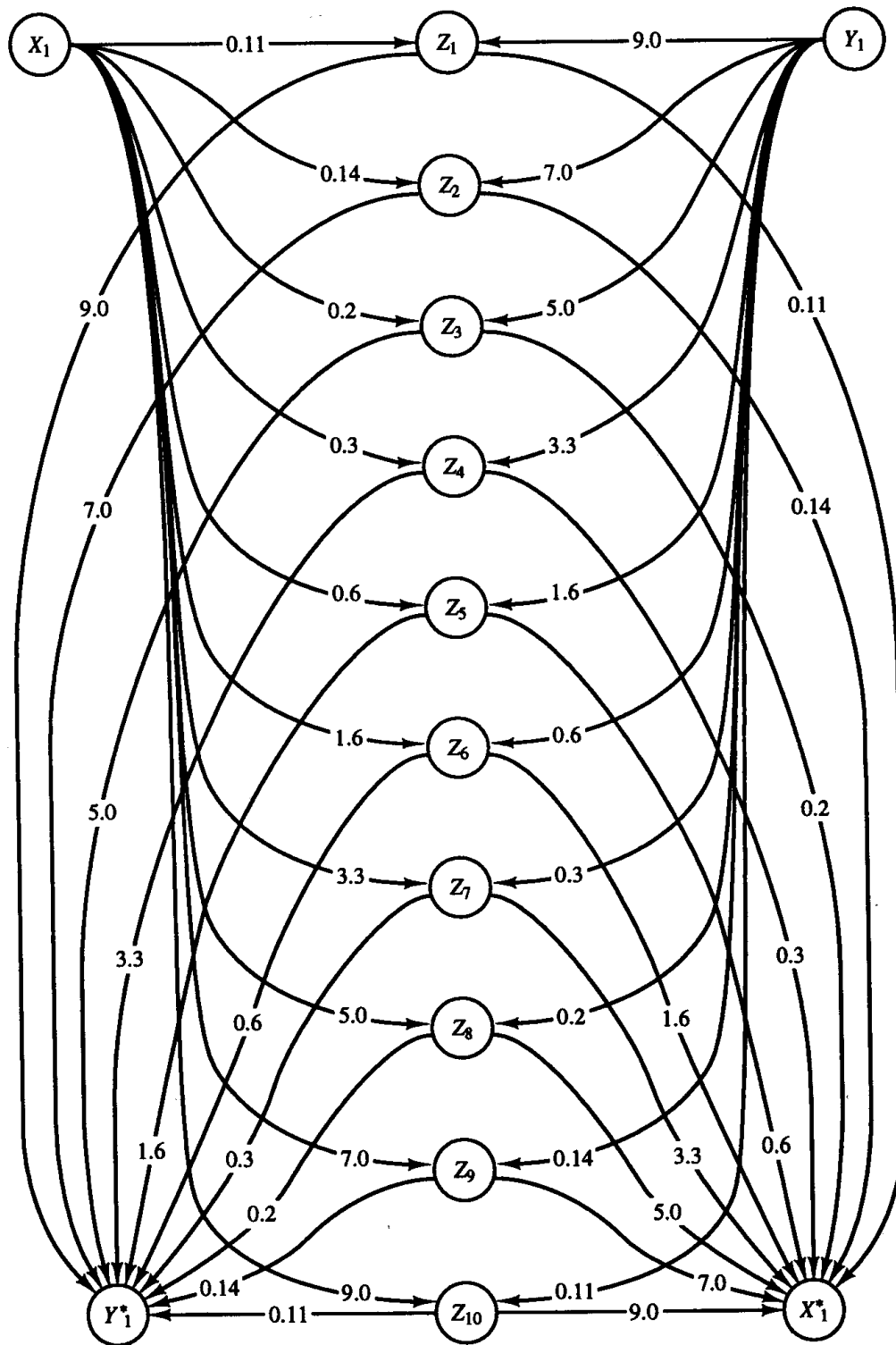
Figure 4.44 Full counterpropagation network for y = 1/x .
