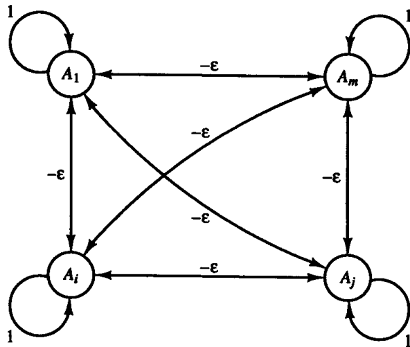
Figure 1.6 Competitive layer.
