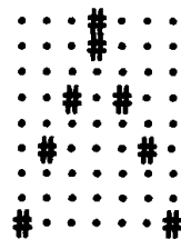
Cluster 1
