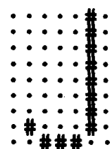
Cluster 4
