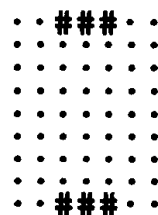
Cluster 3
