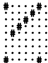
Cluster 5
