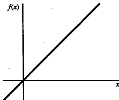
Figure 1.7 Identity function.
