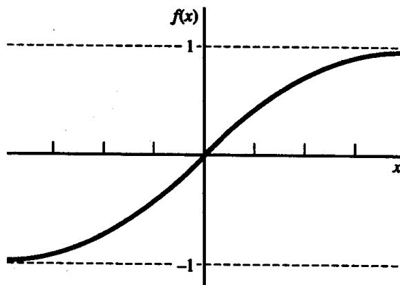
Figure 1.10 Bipolar sigmoid.
