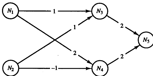
Figure 1.25 Neural network for Exercise 1.1.
