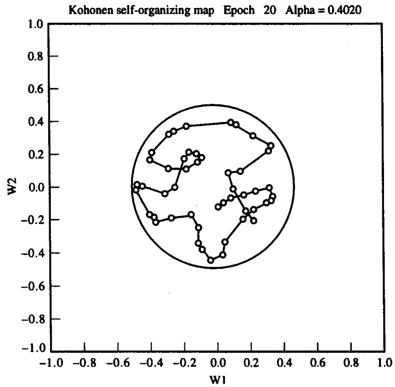
Figure 4.21 Cluster units after 20 epochs.
