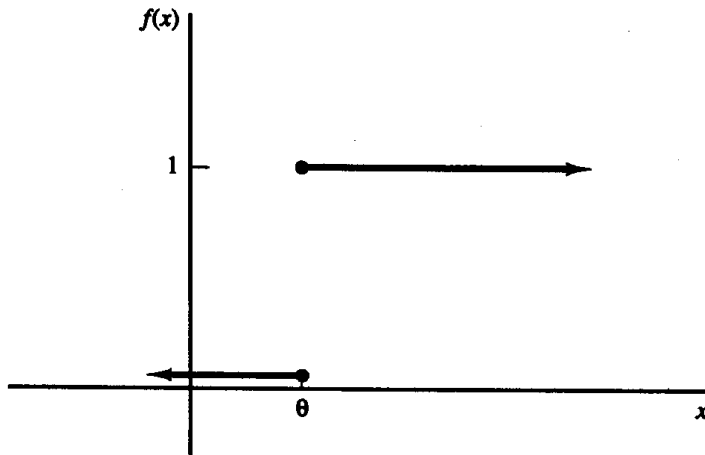
Figure 1.8 Binary step function.
