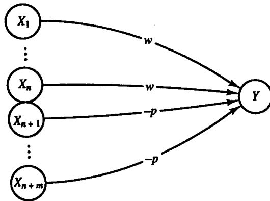
Figure 1.13 Architecture of a McCulloch-Pitts neuron Y .
