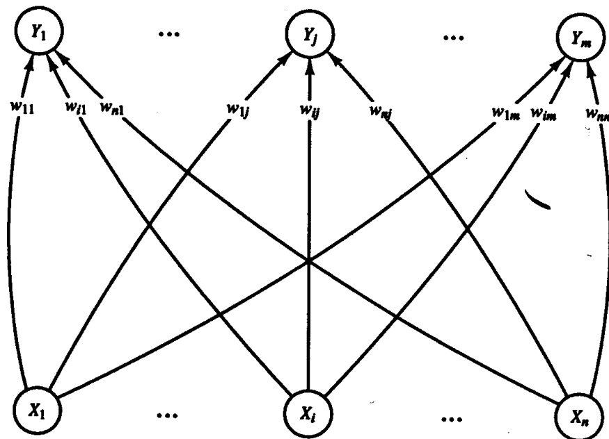
Figure 4.27 Learning vector quantization neural net.
