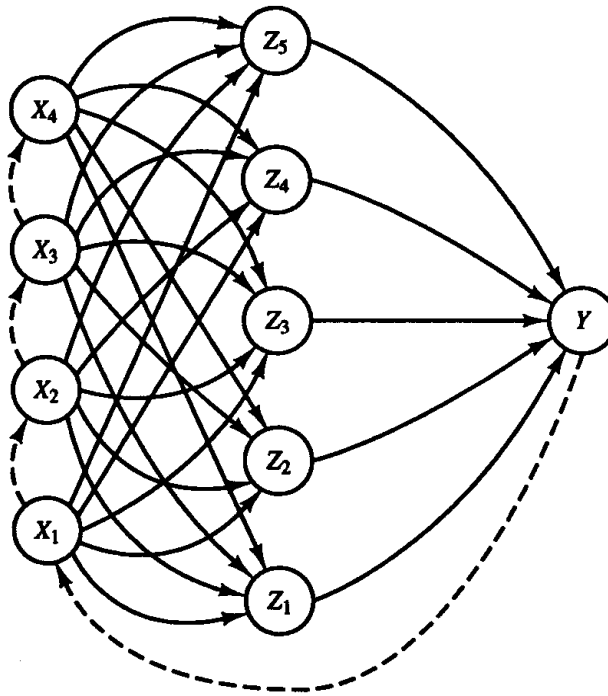
Figure 7.22 Recurrent neural net.
