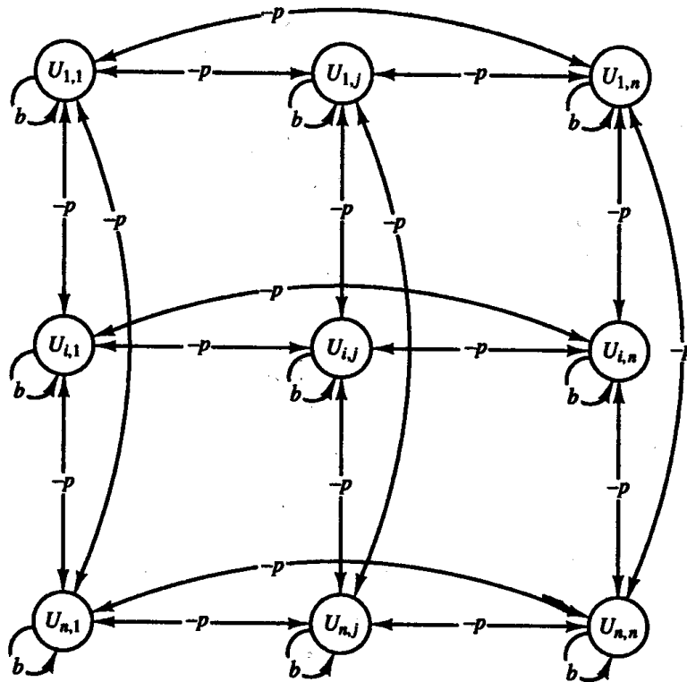
Figure 7.3 Architecture for Boltzmann machine.
