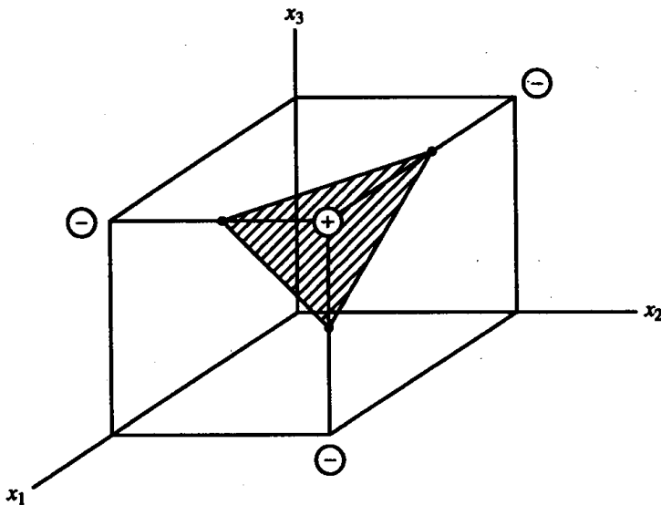
Figure 2.12 Linear separation of binary training inputs.
