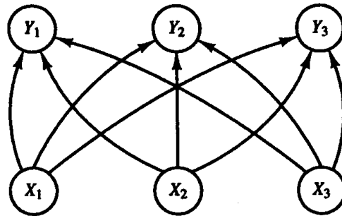
Figure 7.19 Recurrent net used as shift register.
