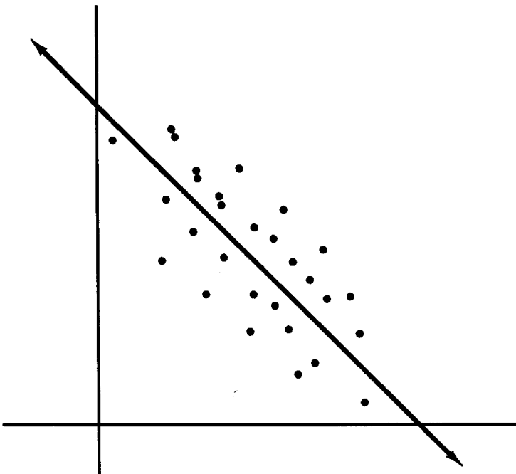
Figure 7.11 Line of best fit.
