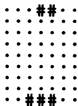
Cluster 2
