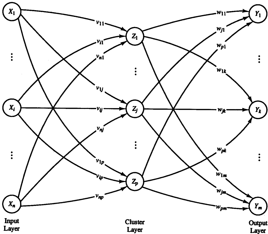
Figure 4.46 Forward-only counterpropagation.
