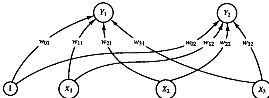
Figure 7.24 Cascade correlation net, Stage 0: No hidden units.
