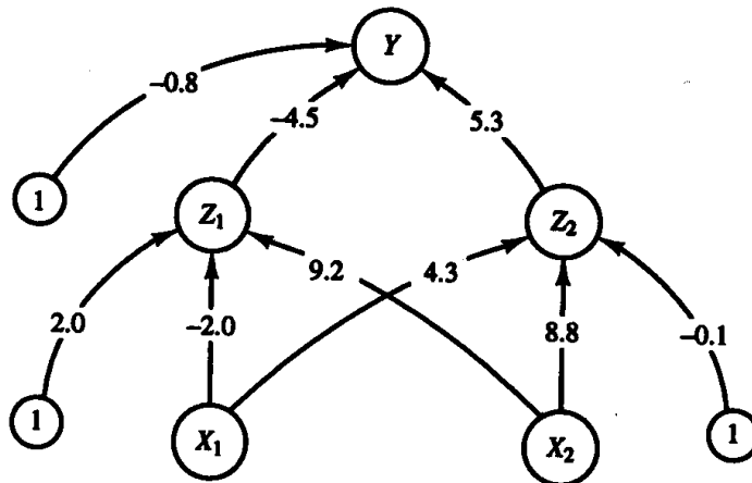
Figure 6.13 Neural network for Exercise 6.6.
