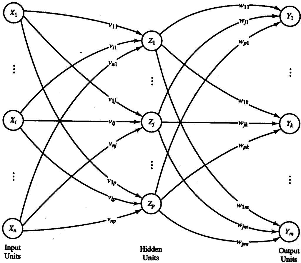
Figure 1.5 A multilayer neural net.
