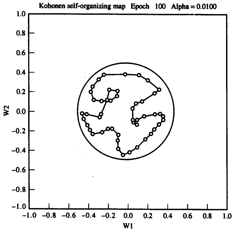
Figure 4.23 Cluster units after 100 epochs.
