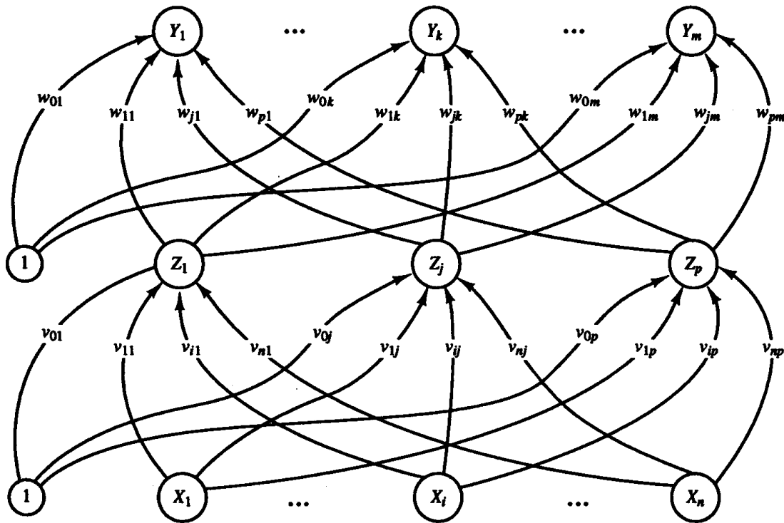
Figure 6.1 Backpropagation neural network with one hidden layer.
