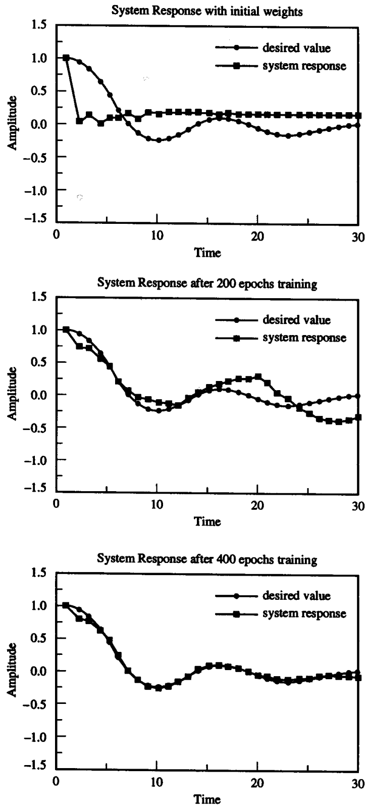
Figure 7.21 Target function and computed response during training.
