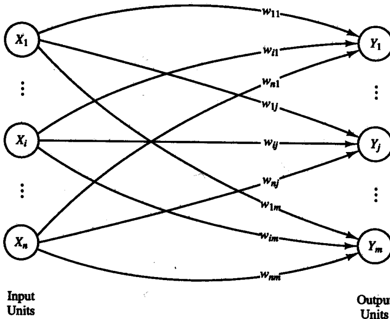
Figure 3.1 Heteroassociative neural net.
