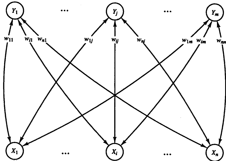
Figure 3.8 Bidirectional associative memory.
