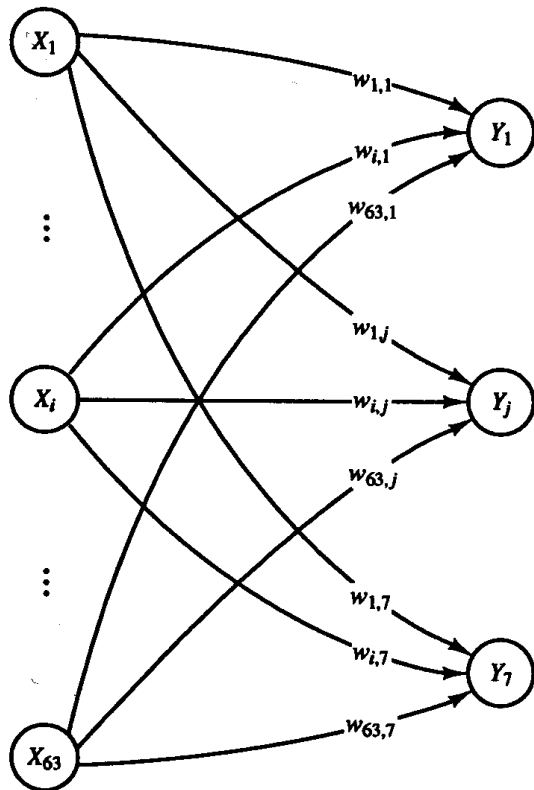
Figure 2.21 Perceptron to classify input into seven categories.
