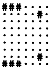
Cluster 6
