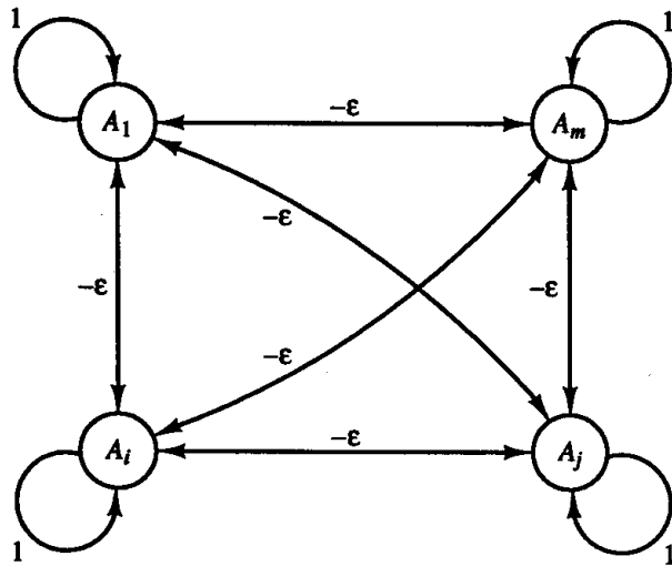
Figure 4.1 MAXNET.
