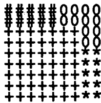
Figure 4.28 Training data
