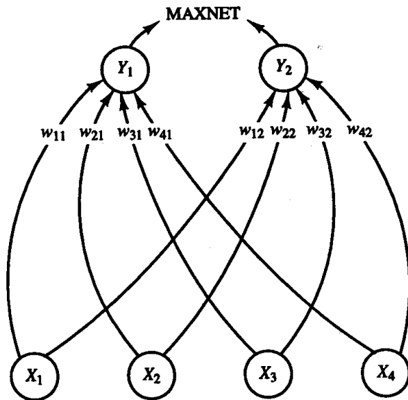
Figure 4.4 Hamming net.
