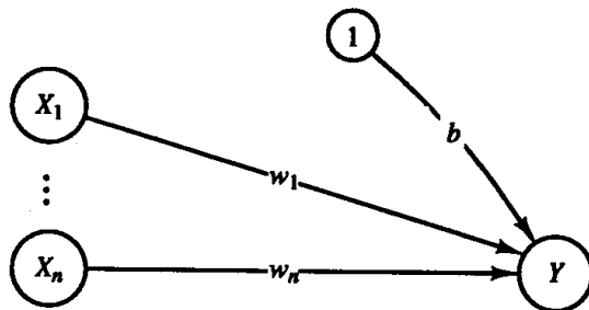
Figure 2.23 Architecture of an ADALINE.
