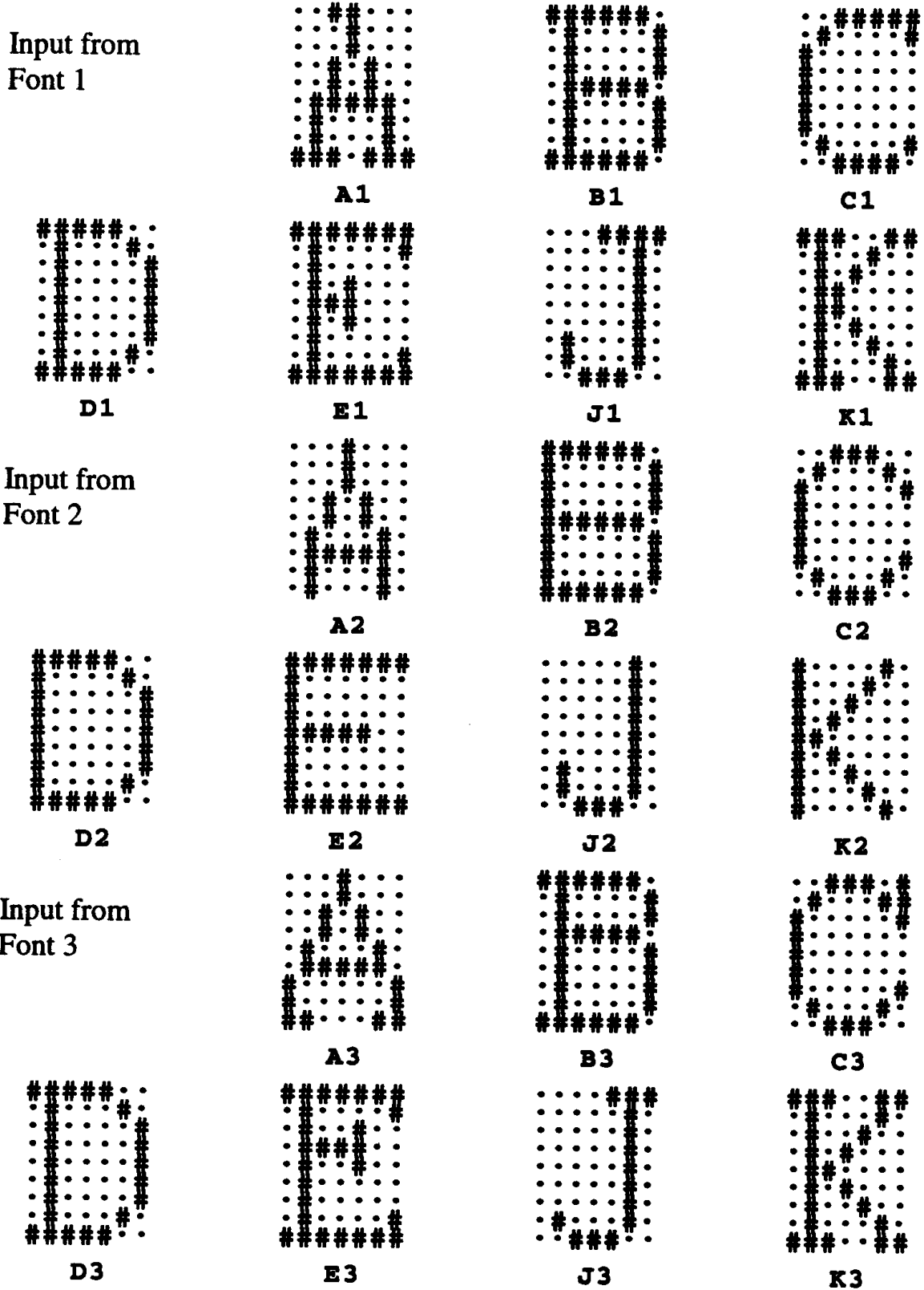
Figure 4.9 Training input patterns for character recognition examples.
