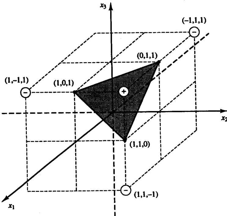
Figure 2.13 Linear separation of bipolar training inputs.
