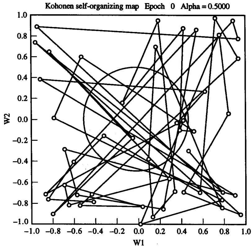
Figure 4.19 Initial cluster units.
