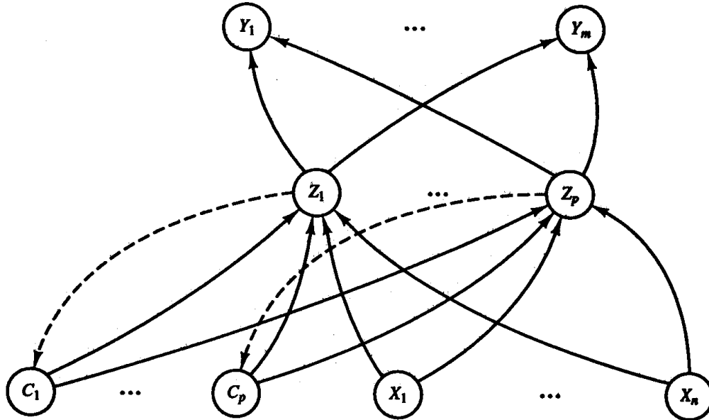
Figure 7.13 Architecture for simple recurrent net.
