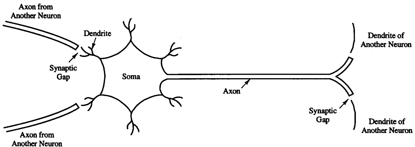
Figure 1.3 Biological neuron.
