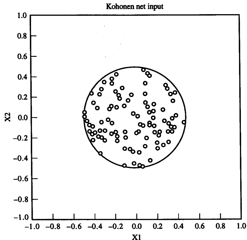
Figure 4.18 Input patterns.
