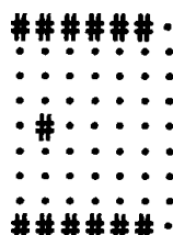
Cluster 7
