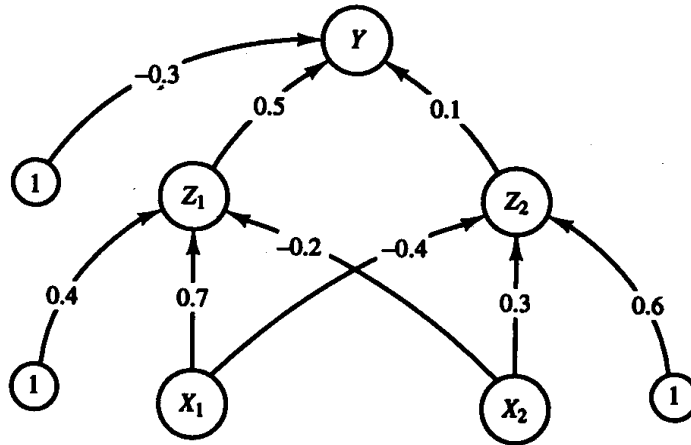
Figure 6.12 Neural network for Exercises 6.1–6.5.
