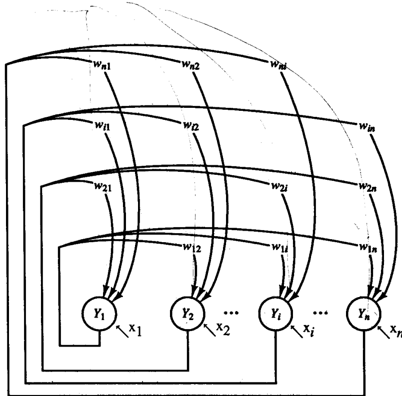
Figure 3.7 Discrete Hopfield net.
