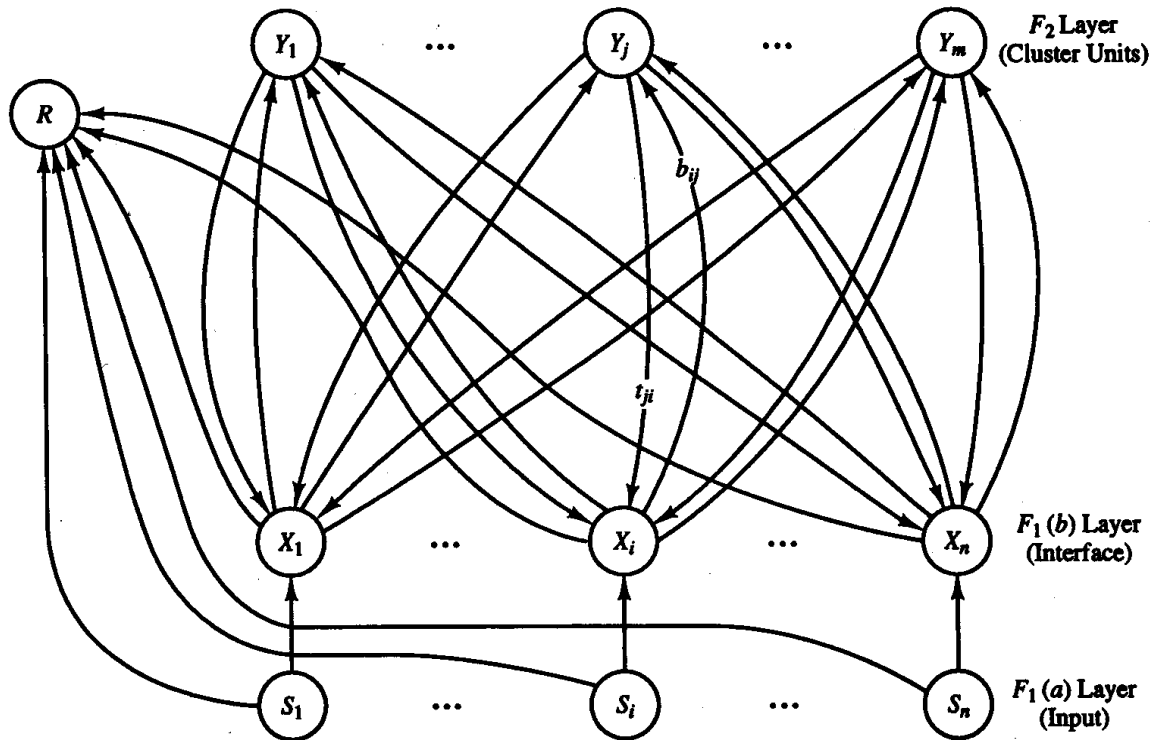
Figure 5.1 Basic structure of ART1.
