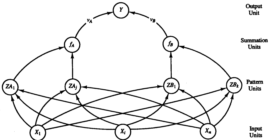
Figure 7.23 Probabilistic neural net.
