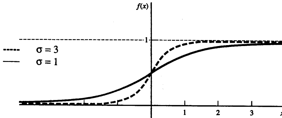
Figure 1.9 Binary sigmoid. Steepness parameters \sigma = 1 and \sigma = 3 .
