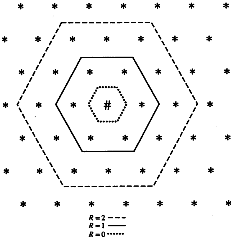
Figure 4.8 Neighborhoods for hexagonal grid.
