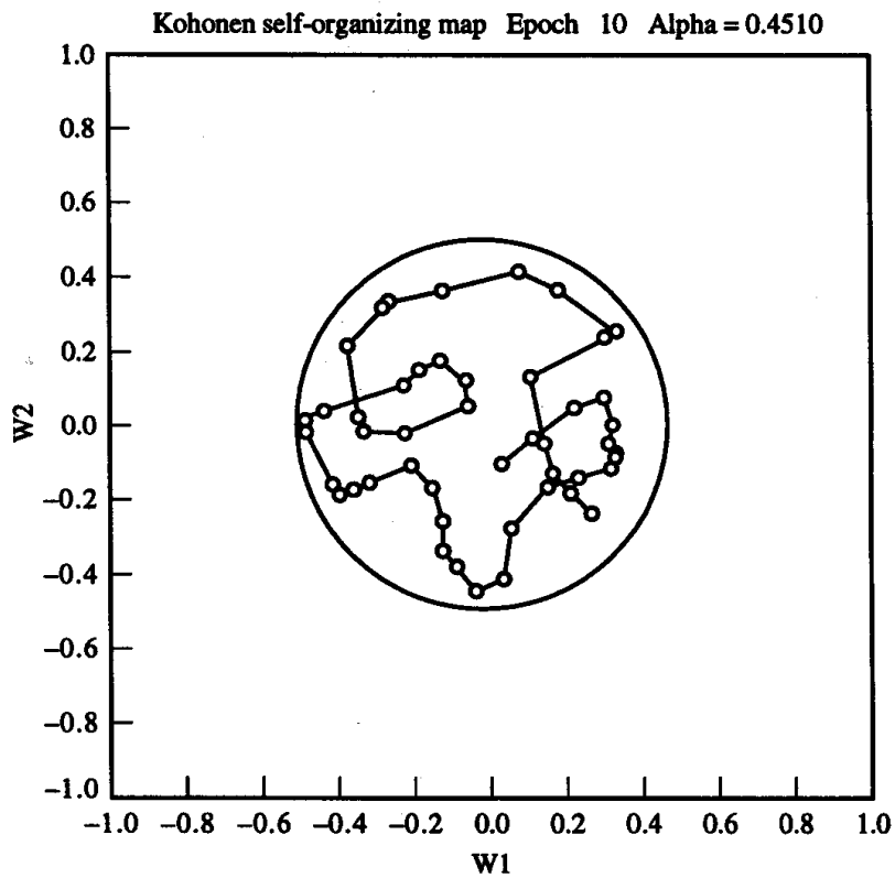
Figure 4.20 Cluster units after 10 epochs.
