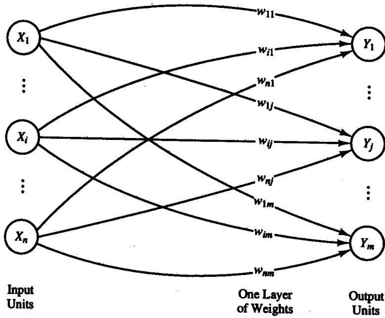
Figure 1.4 A single-layer neural net.
