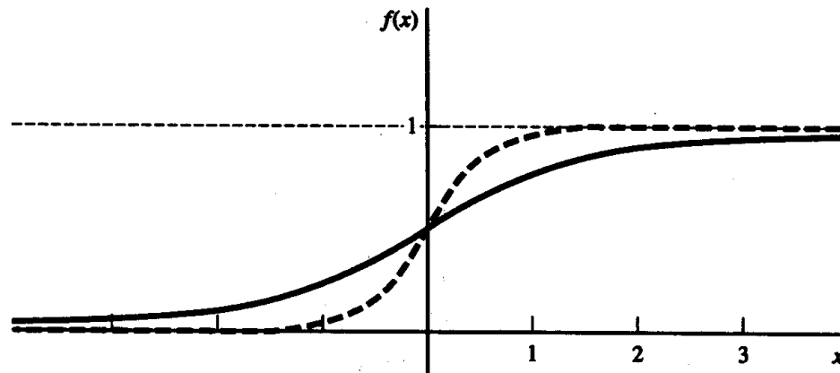
Figure 6.8 Binary sigmoid with \sigma = 1 and \sigma = 3 .
