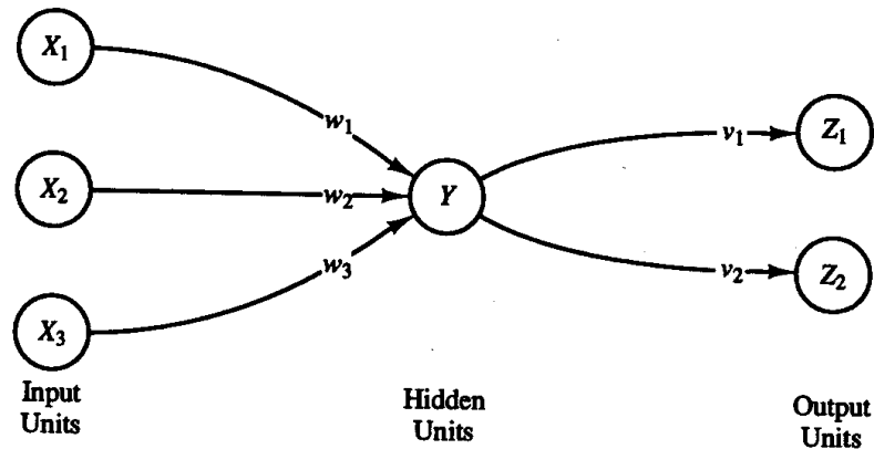
Figure 1.2 A very simple neural network.
