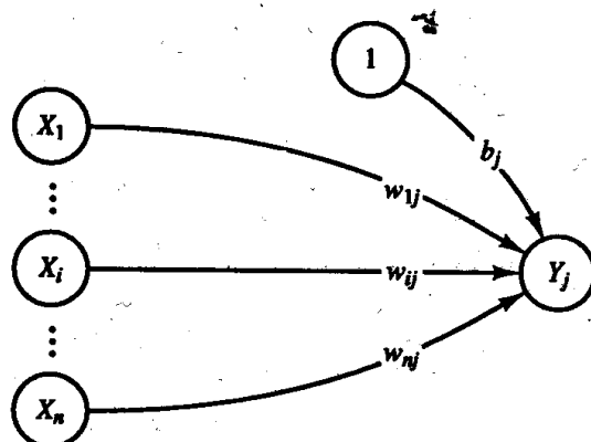
Figure 1.11 Neuron with a bias.
