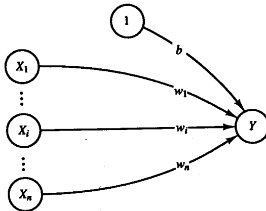
Figure 2.14 Perceptron to perform single classification.
