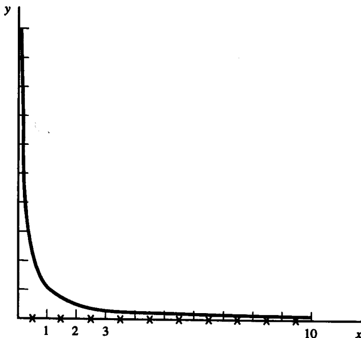
Figure 4.47 Results for y = 1/x using forward-only counterpropagation.
