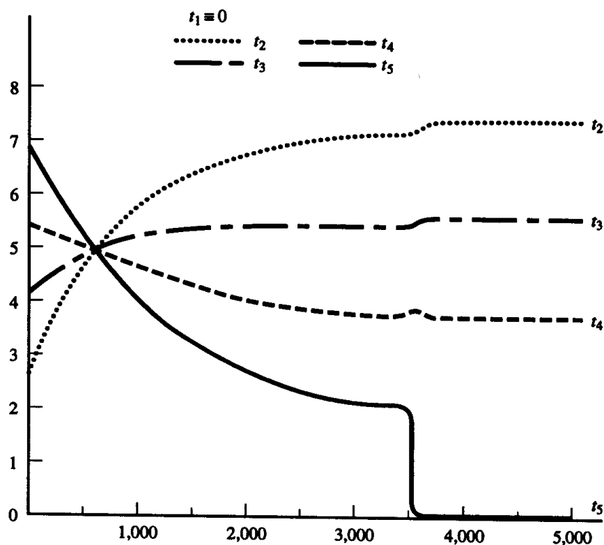
Figure 5.9 Weight changes for Example 5.10.
