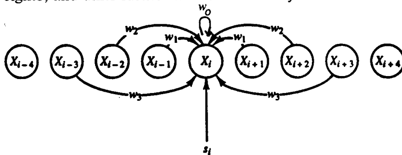
Figure 4.2 Mexican Hat interconnections for unit X_i .
