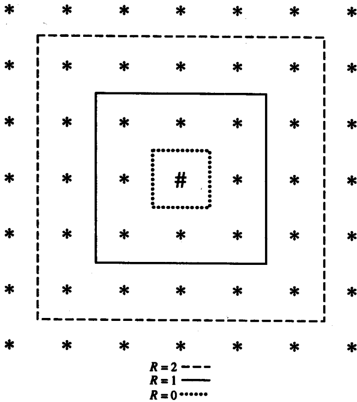
Figure 4.7 Neighborhoods for rectangular grid.
