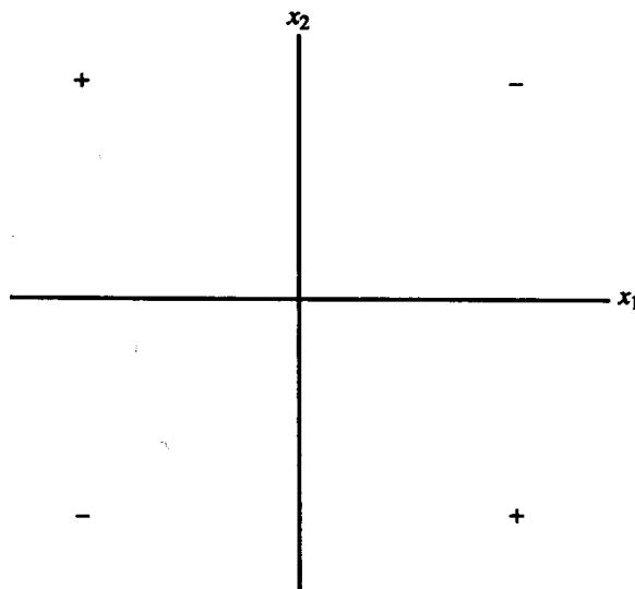
Figure 2.6 Desired response for the logic function XOR.
