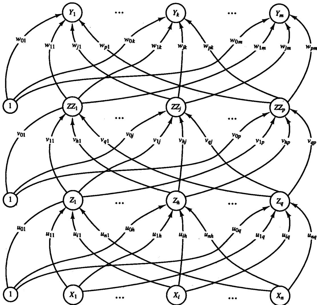
Figure 6.11 Backpropagation neural network with two hidden layers.
