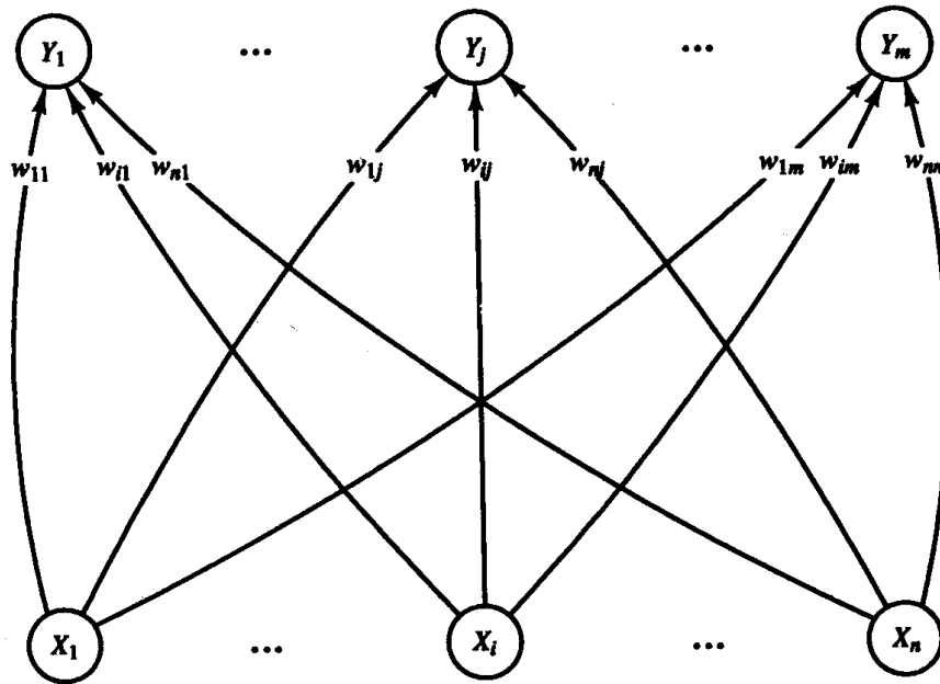
Figure 4.5 Kohonen self-organizing map.
