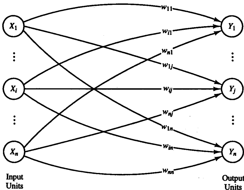
Figure 3.6 Autoassociative neural net.
