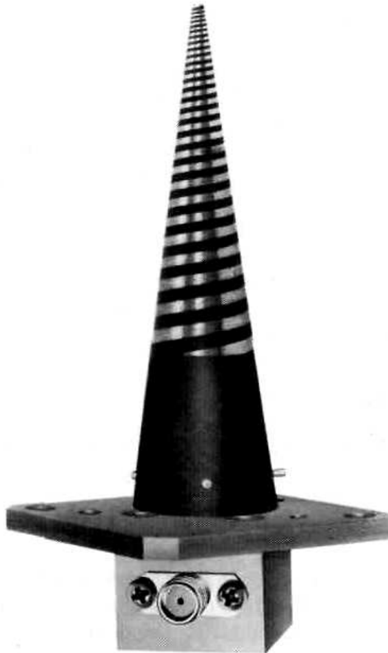
Figure 11.4 Conical spiral metal strip antenna. (SOURCE: Antennas, Antenna Masts and Mounting Adaptors , American Electronic Laboratories, Inc., Lansdale, Pa., Catalog 7.5M-7-79. Courtesy of American Electronic Laboratories, Inc., Montgomeryville, PA 18936 USA)
