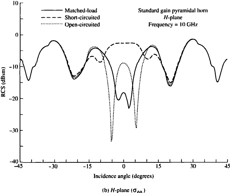
Figure 2.28 E- and H-plane monostatic RCS versus incidence angle for a pyramidal horn antenna.
