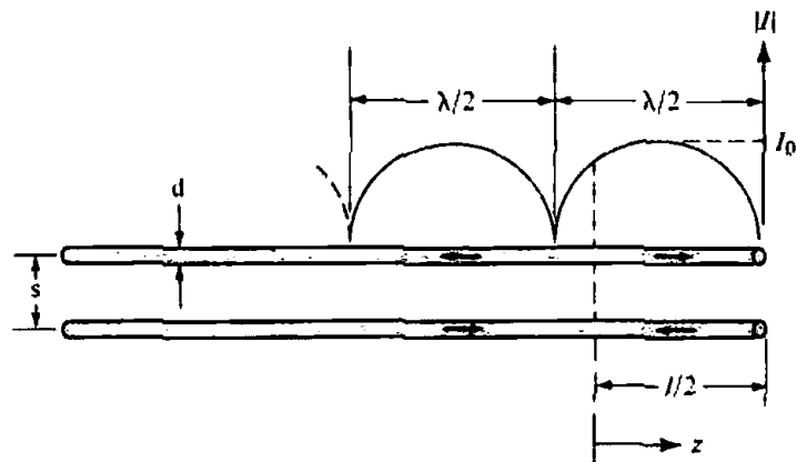
(a) Two-wire transmission line
