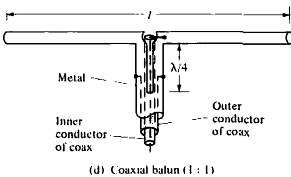
Figure 9.24 Balun configurations.
