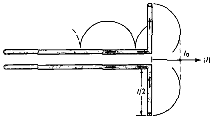
(c) Linear dipole
