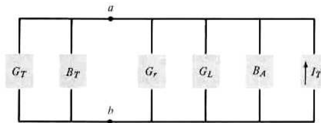
Figure 2.22 Antenna and its equivalent circuits in the receiving mode.
