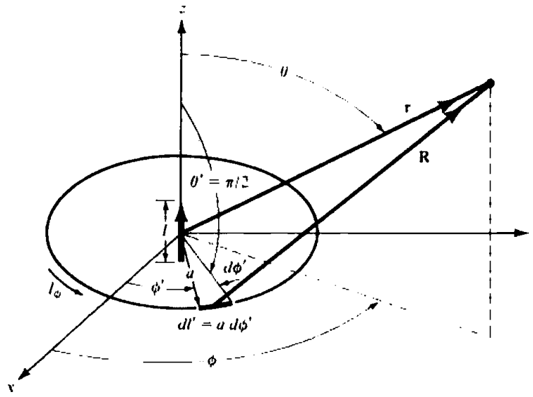
(a) Geometry for circular loop
