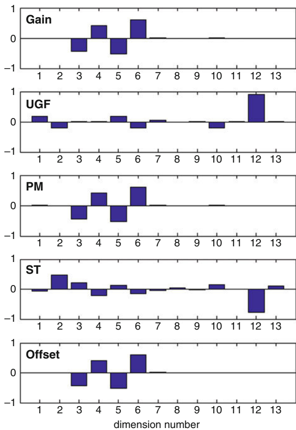
Fig. 16.14 Opamp test case: normalized projection vectors for the first LVs of the opamp metrics: we can see the strong relationship between gain, PM, and offset
