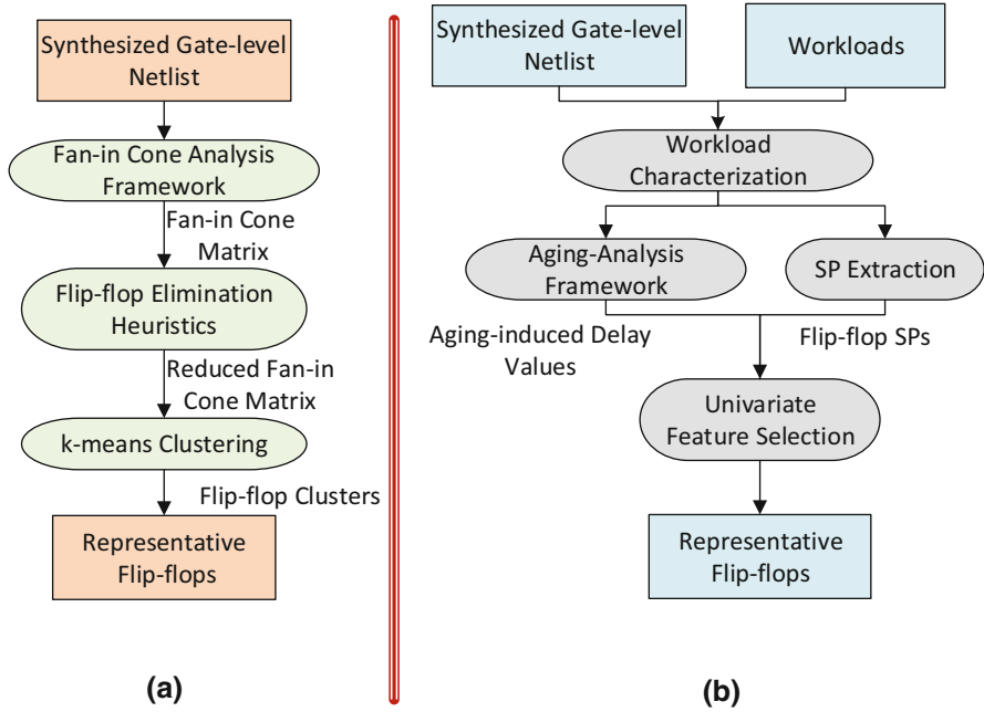
Fig. 9.6 Overall flow of space-sampling techniques to identify representative flip-flops. (a) Fan-in cone-based flip-flop selection. (b) Correlation-based flip-flop selection
