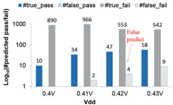
Fig. 11.13 Selective_Boost design Phase 2 pass/fail prediction for the importance sample points. No false passing (false negatives) points were reported for these experiments [8]
