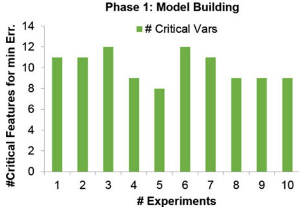
Fig. 11.11 Optimal number of critical features. Experiments 1 through 6 represent Selective_Boost_WA design for V_{dd} range of [0.35–0.40 V]. Experiments 7 to 10 represent the Selective_Boost design for V_{dd} range of [0.40–0.43 V] [8]
