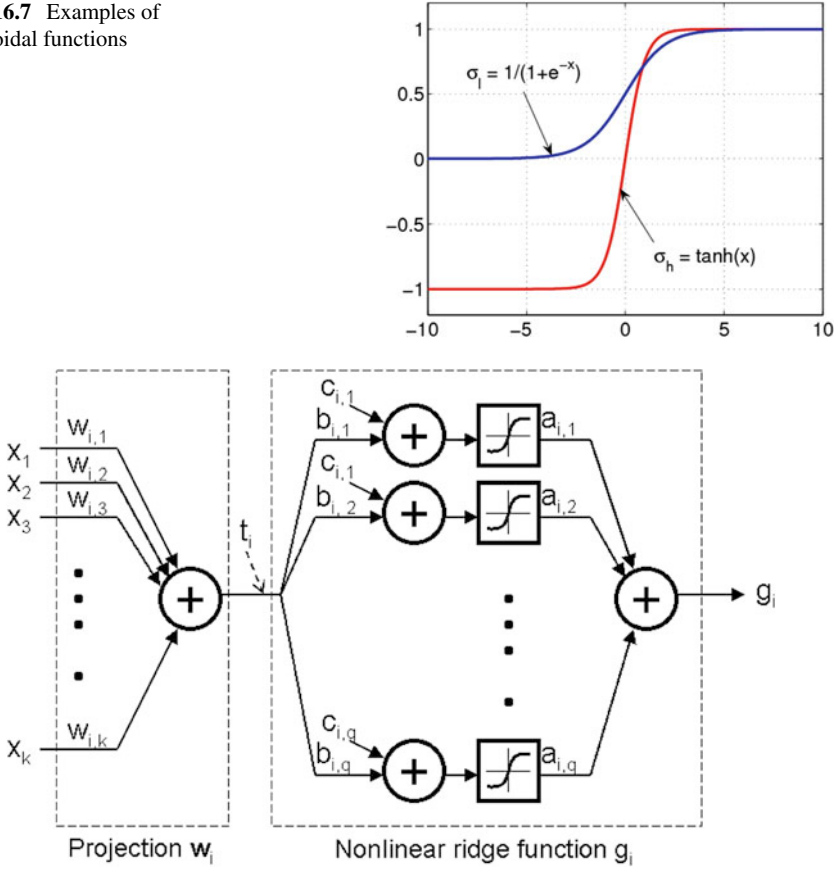
Fig. 16.8 The network corresponding to the i -th component in the SiLVR model (16.54)
