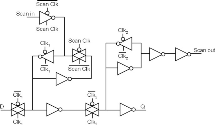
Fig. 16.11 A master–slave flip-flop with the scan chain component
