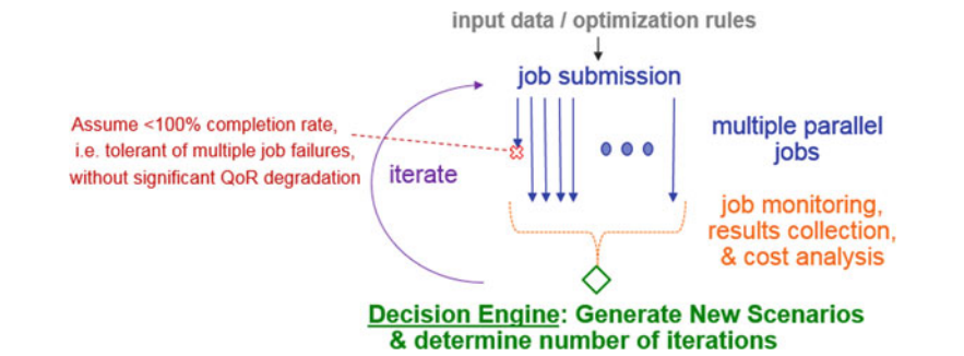
Fig. 18.7 A common compute footprint utilized by SynTunSys decision engines
