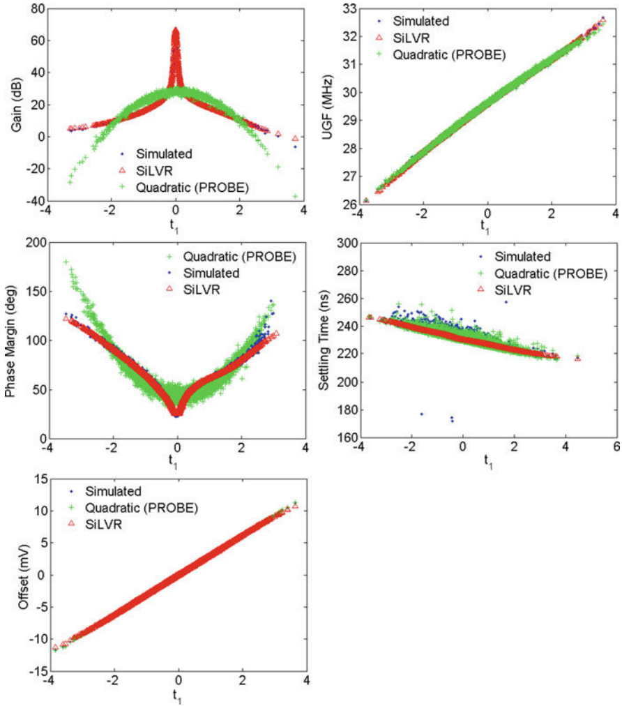
Fig. 16.15 Opamp test case: simulated, PROBE-predicted (green plus), and SiLVR-predicted (red triangle) opamp outputs, plotted against first LV. For the nonlinear cases, the simulated and SiLVR-predicted graphs coincide in many places
