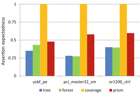
Fig. 20.15 The average normalized expectedness of the assertions that passed formal verification for each data mining algorithm
