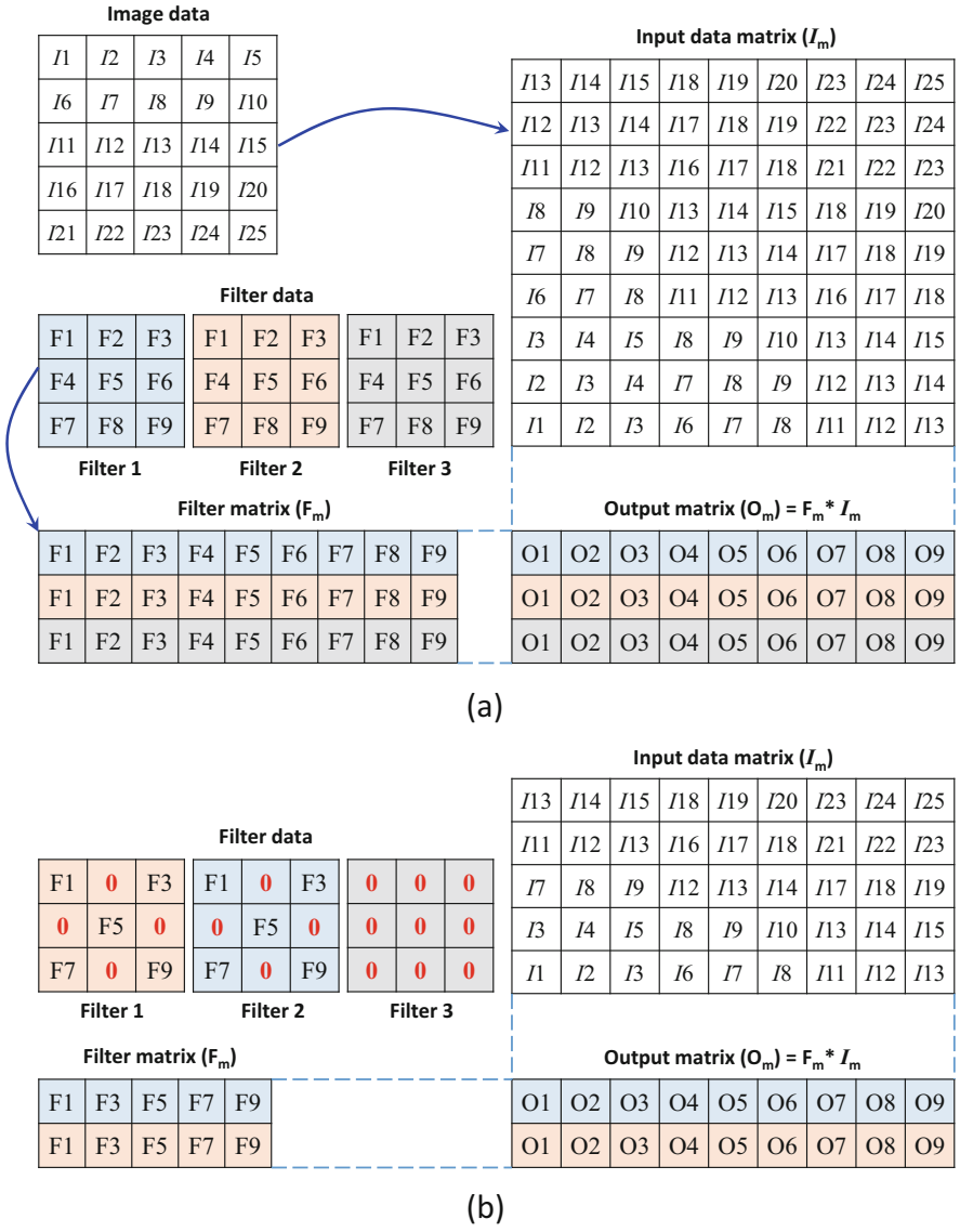
Fig. 21.5 Lowering convolution to matrix multiplication for pruned and unpruned networks. (a) illustrates the conversion of input data and filters into matrices that can be multiplied to generate the resultant output. (b) shows the reduction in the dimensions of matrices in case of structured pruning
