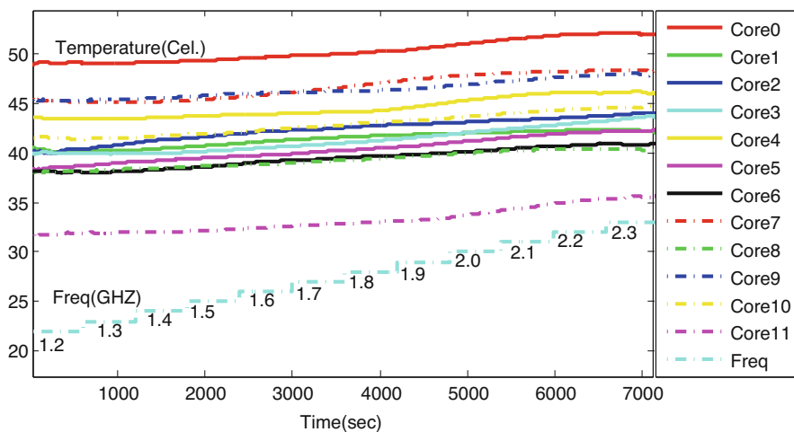
Fig. 19.11 Per-core temperature vs. frequency and time plot for 12 cores
