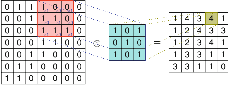
Fig. 4.4 Example of convolution with one kernel filter
