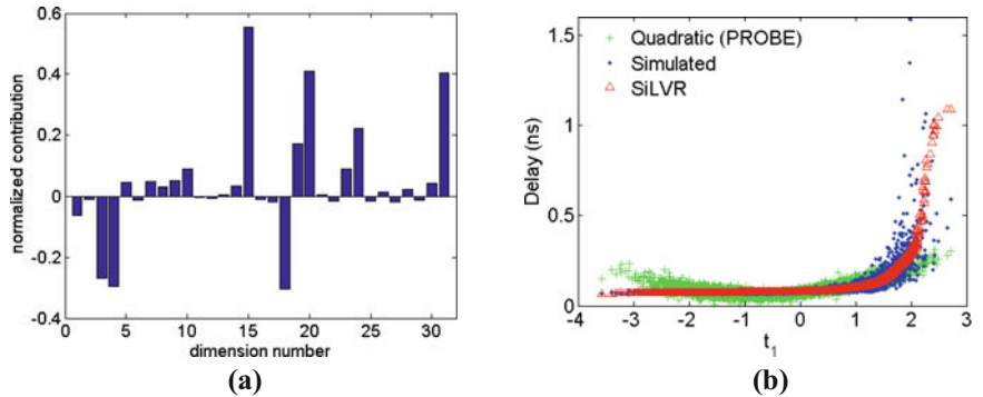
Fig. 16.12 Performance of SiLVR on the MSFF test case. (a) The normalized projection weights for the first LV. (b) Simulated, SiLVR-predicted (red triangle), and PROBE-predicted (green plus) delay values, plotted against the first LV
