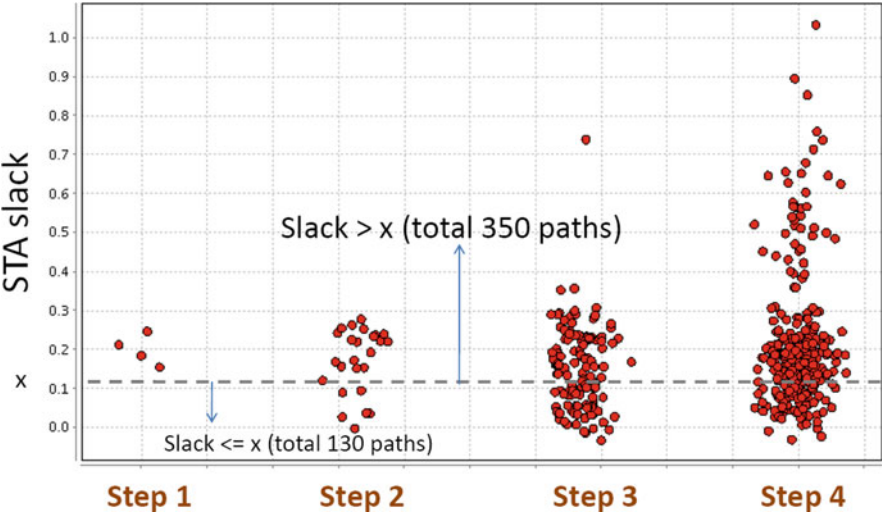
Fig. 13.4 350 critical paths not predicted by STA
