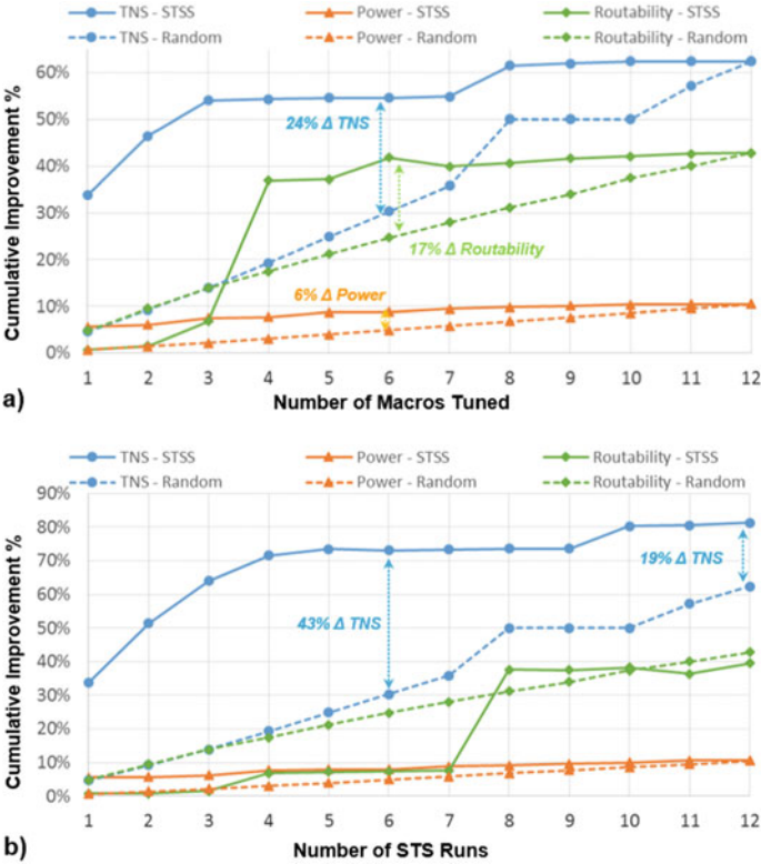
Fig. 18.24 Results of tuning 12 macros based on STSS priority ordering vs. random ordering. (a) Priority ranked tuning vs. random tuning. (b) Priority ranked tuning vs. random tuning, allowing second pass tuning runs
