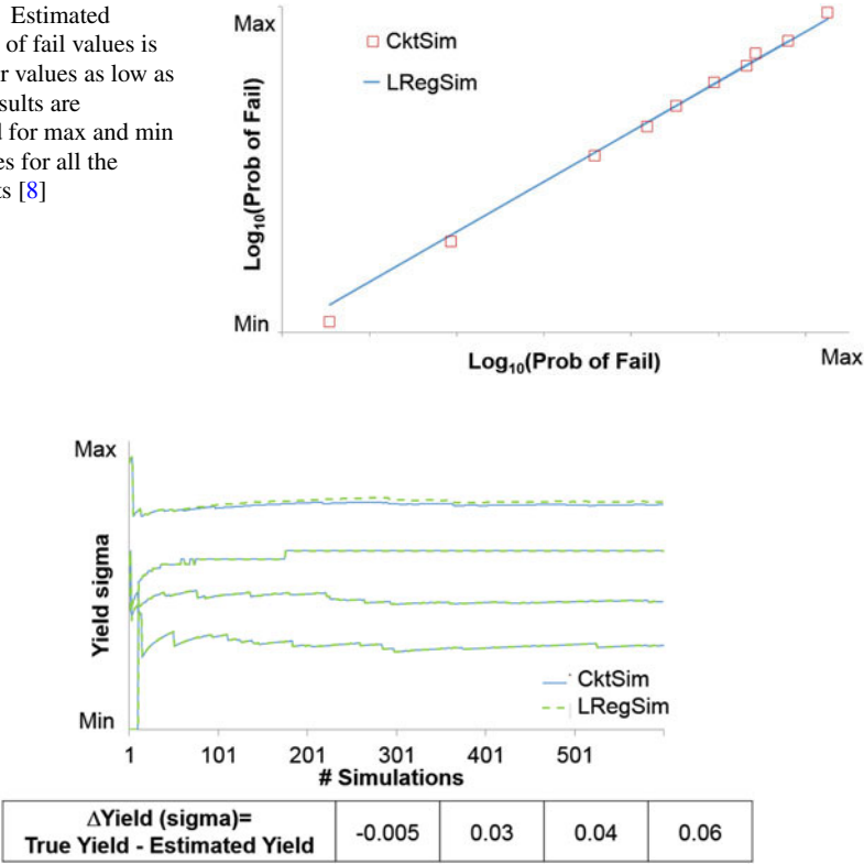
Fig. 11.17 Selective_Boost design yield prediction. Results are normalized for max and min yield. True yield refers to CktSim approach, and estimated yield to LRegSim [8]
