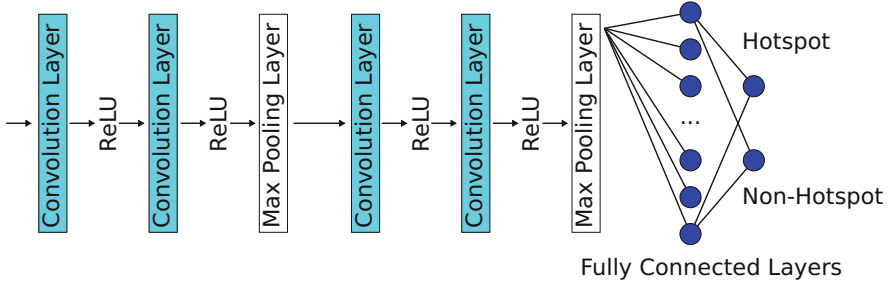
Fig. 4.5 An example of a neural network for hotspot detection [54]
