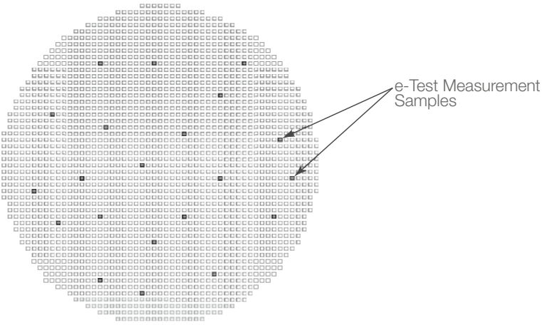
Fig. 5.15 e-Test measurements
