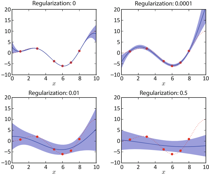
Fig. 5.4 Effects of the regularization parameter when learning from training data
