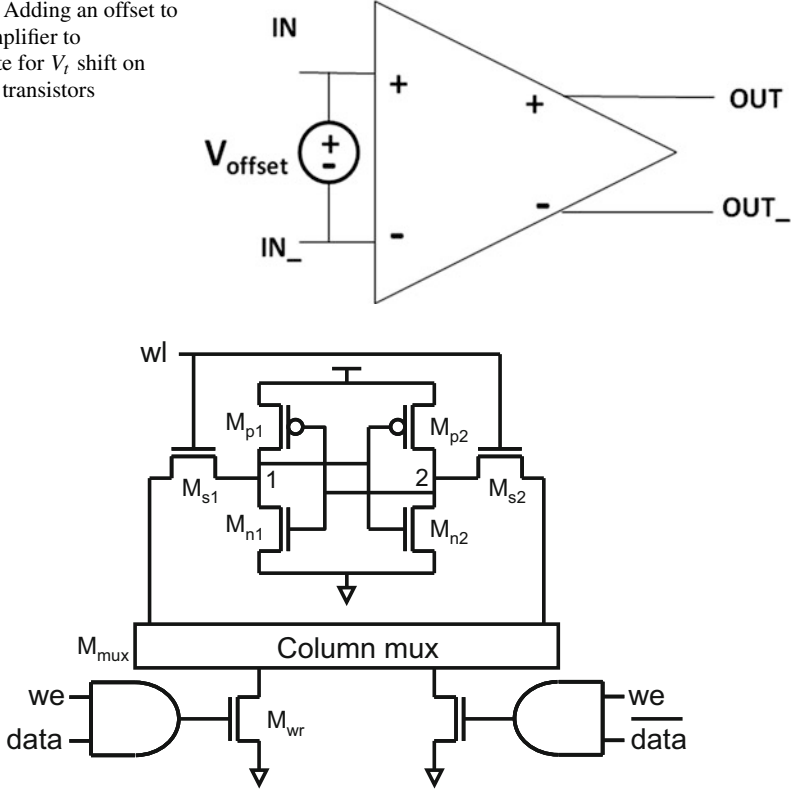
Fig. 10.9 A 6-transistor SRAM cell with write driver and column mux
