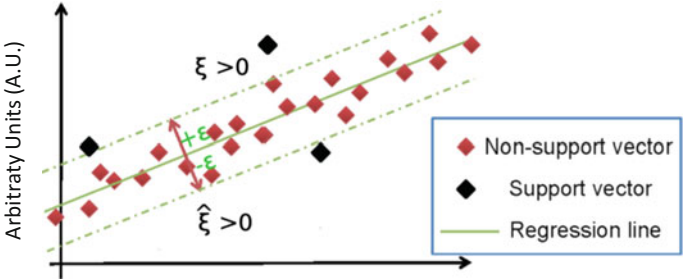
Fig. 9.5 Illustration of the support-vector regression model
