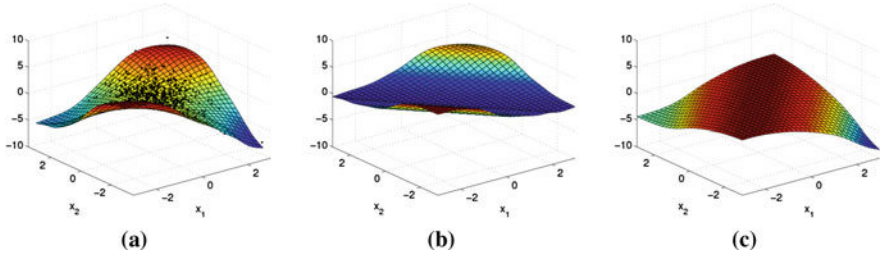
Fig. 16.10 A 2-LV SiLVR model for y = x_1x_2 for (x_1, x_2) \sim \mathcal{N}(\mathbf{0}, \mathbf{I}_2) . (a) The surface extracted by a 2-LV SiLVR model, and the training samples. (b) The first ridge function g_1 extracted by SiLVR, along \mathbf{w}_1 = (0.7285, 0.6851) . (c) The second ridge function g_2 extracted by SiLVR, along \mathbf{w}_2 = (0.7296, -0.6838)
