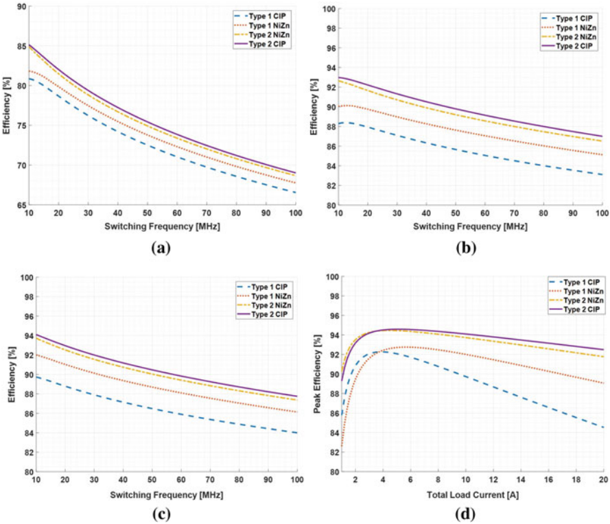
Fig. 17.12 Efficiency comparison of four optimized IVRs as a function of switching frequency and total load current. (a) 5 V:1 V conversion ( I_{LOAD} = 10 A). (b) 3 V:1 V conversion ( I_{LOAD} = 10 A). (c) 1.7 V:1.05 V conversion ( I_{LOAD} = 10 A). (d) Eff. vs. load current ( f_{SW} = 10 MHz)
