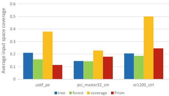
Fig. 20.10 The average input space coverage of generated assertions for each data mining algorithm
