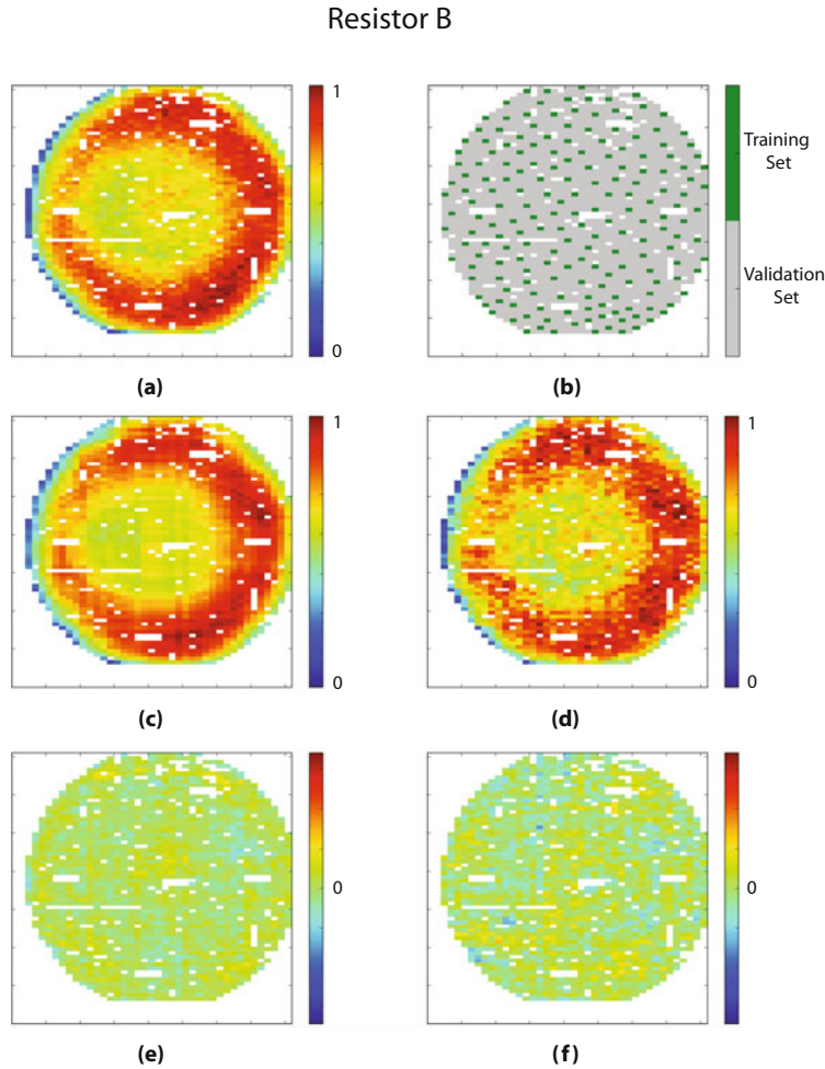
Fig. 5.29 Actual and predicted lengths using both methods for resistor B. (a) Actual trim length. (b) Sampled locations. (c) Length-based, original target predicted length. (d) Rate-based, original target predicted length. (e) Length-based, original target prediction error. (f) Rate-based, original target prediction error
