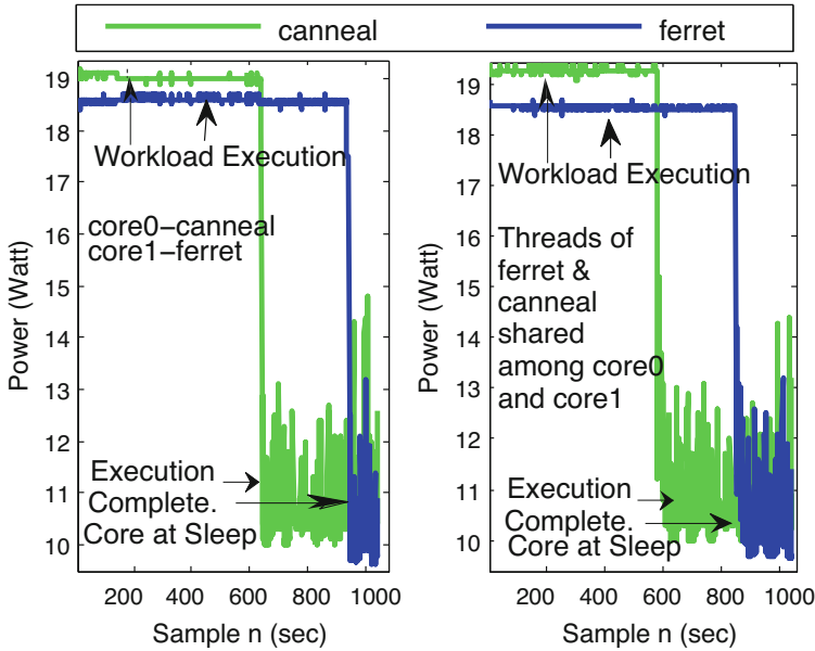
Fig. 19.23 Power and runtime comparison for thread swapping across workload
