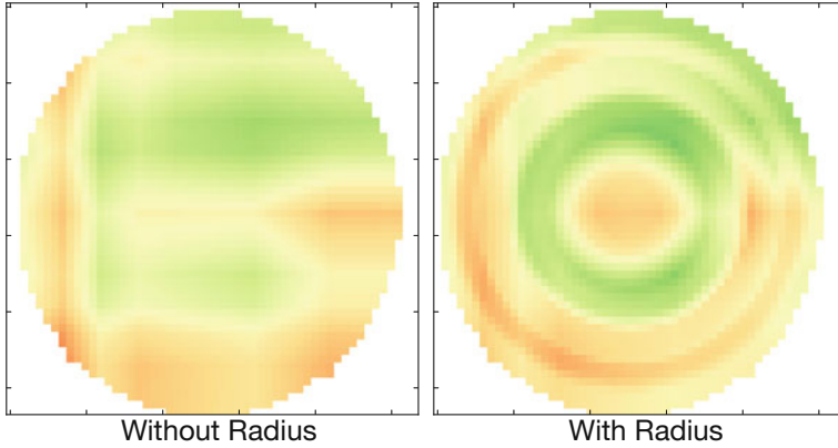
Fig. 5.6 Radial modeling
