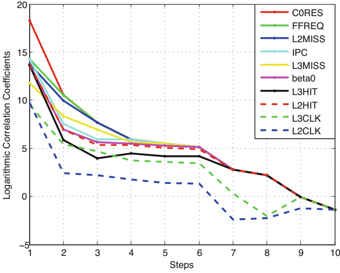
Fig. 19.3 Correlation coefficients of PCs with power
