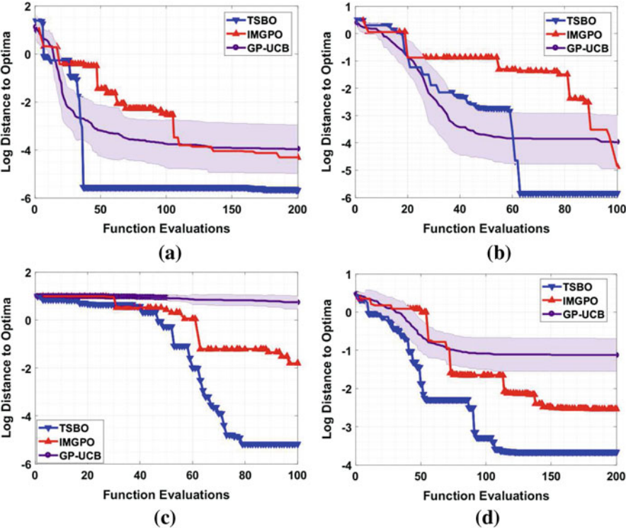
Fig. 17.7 Performance comparison for proposed algorithm, TSBO, on optimization challenge functions used in the literature. Functions are available in [19]. (a) 2D Branin function. (b) 3D Hartmann function. (c) 4D Shekel5 function. (d) 6D Hartmann function
