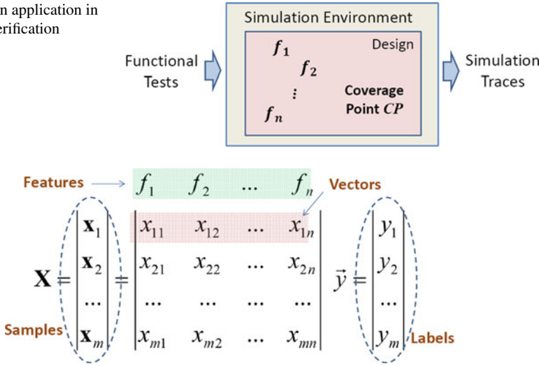
Fig. 13.2 The format of a dataset to be analyzed
