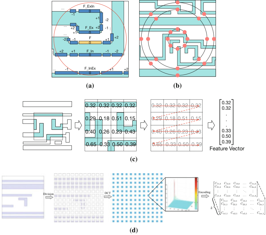
Fig. 4.2 (a) Fragmentation based hotspot signature extraction [8]. (b) CCAS feature extraction [23]. (c) Density-based pattern representation [60]. (d) Feature tensor generation [54]
