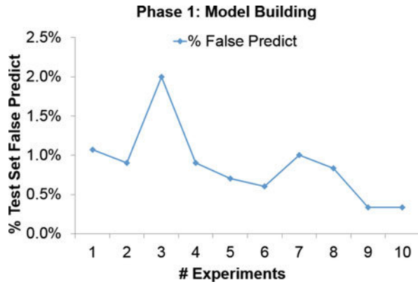
Fig. 11.12 Test set prediction error corresponding to the model based on the critical number of variables in Fig. 11.11. Experiments 1 through 6 represent Selective_Boost_WA design for V_{dd} range of [0.35–0.40 V]. Experiments 7 to 10 represent the Selective_Boost design for V_{dd} range of [0.40–0.43 V] [8]
