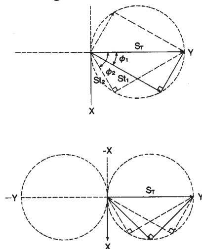
Figure 17.3.8: Typical transverse sensitivity plot.
