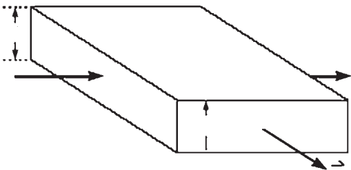
Figure 15.3.9: Hall effect sensors.
