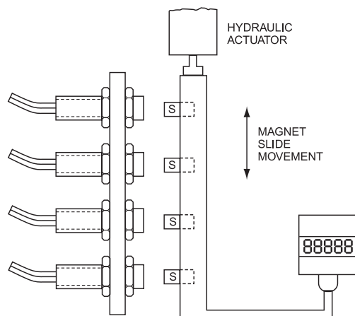
Figure 15.1.14: Four digital output, unipolar sensors are threaded into an aluminum housing and actuated individually by four magnetic actuators.
