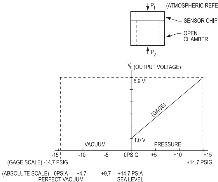
Figure 16.1.3: A high-level gauge pressure sensor output is shown. One-volt output represents ambient pressure.
