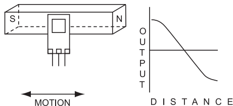
Figure 15.1.19: Slide-by position sensor.
