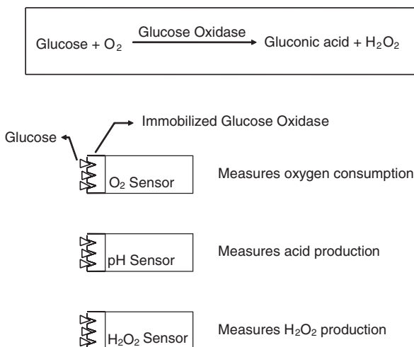
Figure 6.1.3: Three possible transducers for glucose measurement.
