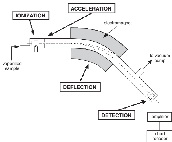
Figure 7.1.4: Mass spectrometer.
