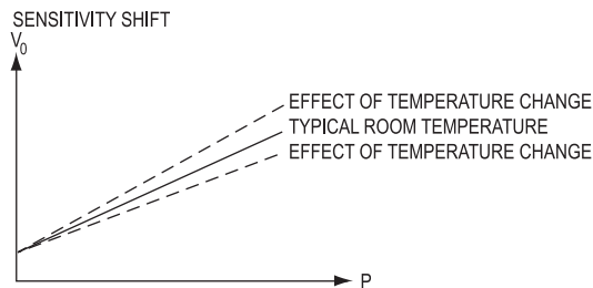
Figure 16.1.13: Sensitivity shift error.
