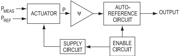
Figure 16.1.18: Auto-reference with reference condition actuators.
