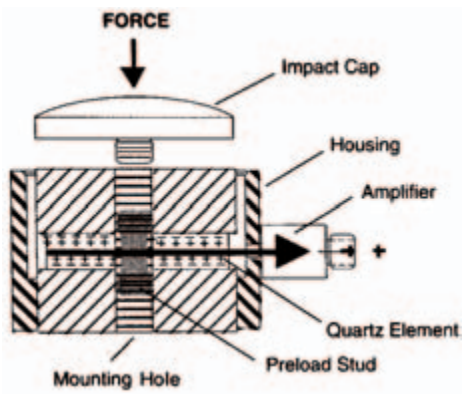
Figure 11.2.5: Cross section of a general purpose force sensor.
