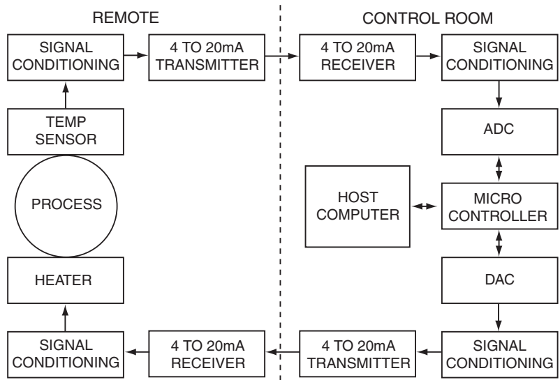
Figure 1.2.3: Typical industrial process control loop.
