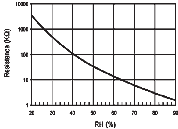
Figure 12.2.2: Relationship of impedance change to humidity. Source: Roveti, Denes. "Choosing a Humidity Sensor: A Review of Three Technologies." Sensors Online. July 2001. http://www.sensorsmag.com/articles/0701/54/main.shtml
