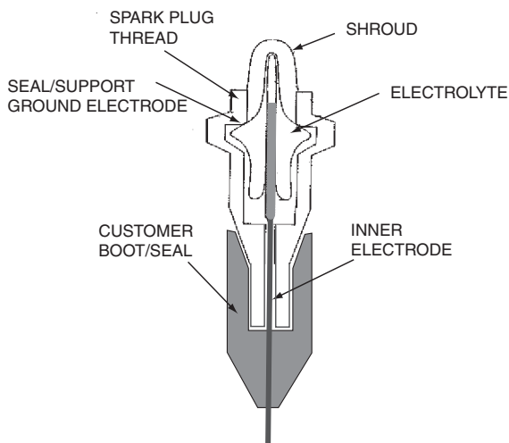
Figure 7.2.1: O 2 sensor.
