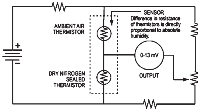
Figure 12.2.3: Thermal conductivity (or absolute) humidity sensors. Source: Roveti, Denes. "Choosing a Humidity Sensor: A Review of Three Technologies." Sensors Online. July 2001. http://www.sensormag.com/articles/0701/54/main.shtml
