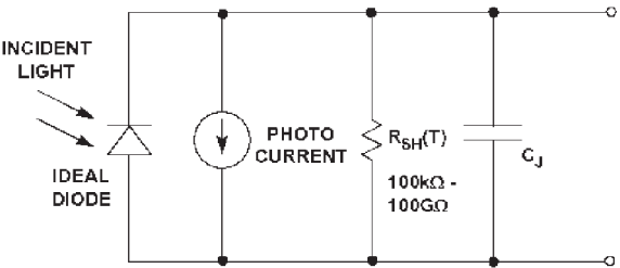
Figure 4.4.2: Photodiode applications.
