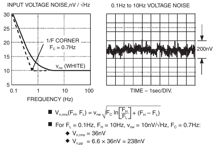
Figure 4.2.9: Input voltage noise for OP177/AD707.
