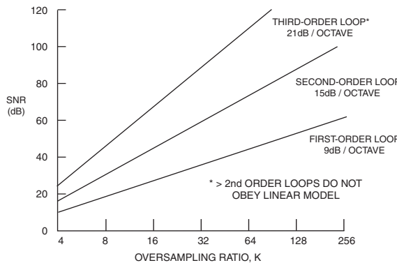
Figure 4.3.20: SNR versus oversampling ratio for first, second, and third-order loops.
