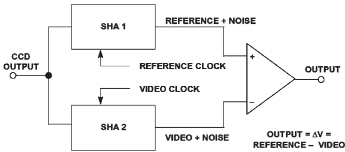
Figure 4.4.39: Correlated double sampling (CDS).
