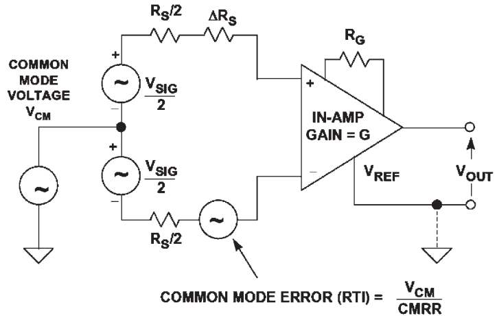
Figure 4.2.25: Instrumentation amplifier.
