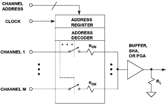
Figure 4.3.12: Simplified diagram of a typical analog multiplexer.
