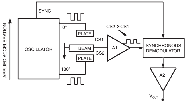
Figure 15.3.20: ADXL-family accelerometers internal signal conditioning.
