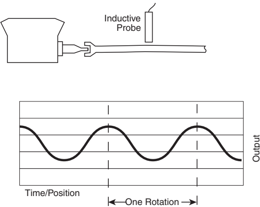
Figure 8.7.18: Inductive sensors are ideal for measuring rotating motion when the environment is dirty and accuracy less than a micron is not required.
