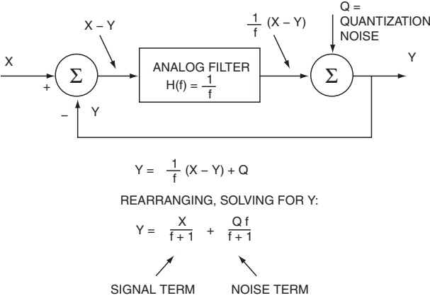
Figure 4.3.17: Simplified frequency domain linearized model of a sigma-delta modulator.
