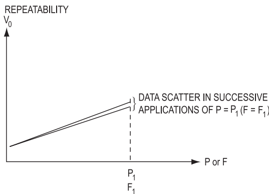
Figure 16.1.10: Repeatability error.
