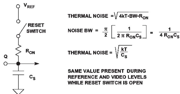
Figure 4.4.38: kT/C noise.
