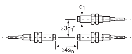
Figure 15.1.45: Minimum mounting distances for unshielded sensors
