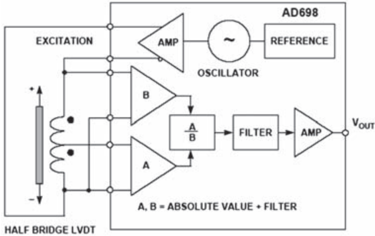
Figure 15.3.8: Half-bridge LVDT configuration.
