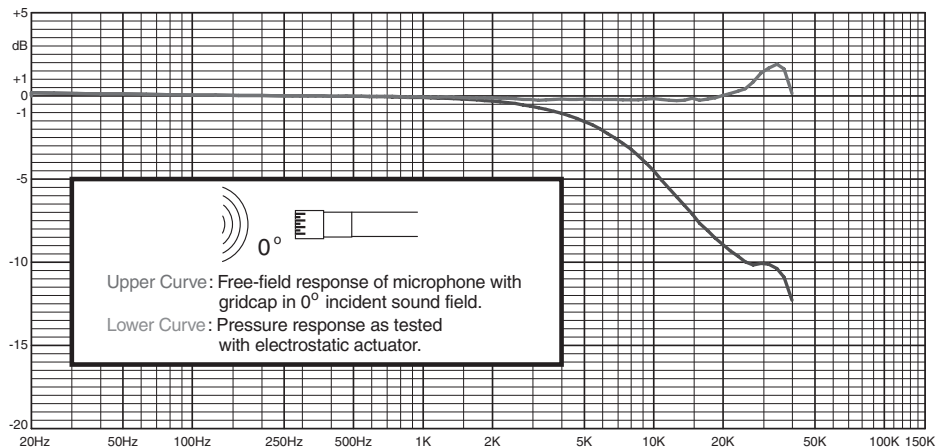
Figure 18.5.4: Free field microphone frequency response.
