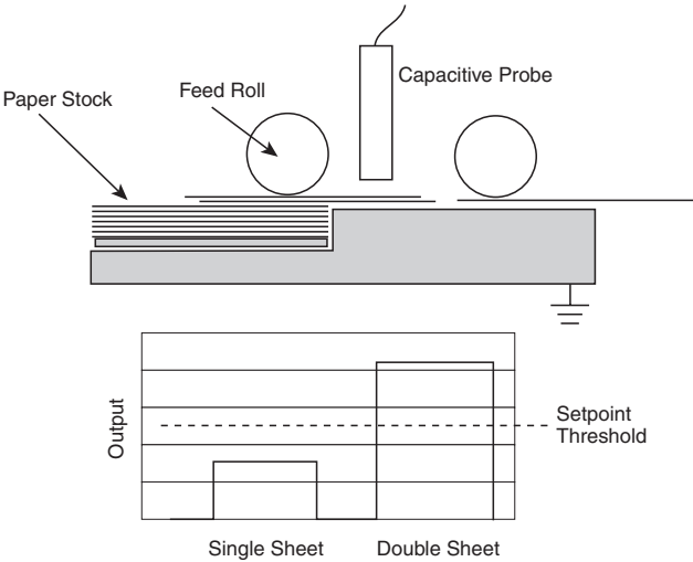
Figure 8.7.15: Capacitive sensors detect increases in the amount of material in the gap such as paper thickness.
