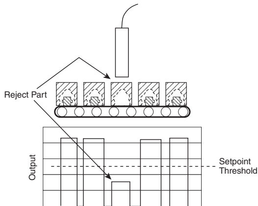
Figure 8.7.8: Incomplete assemblies are detected on a production line by a sensor with a switched output.
