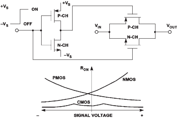
Figure 4.3.11: Basic CMOS analog switch.
