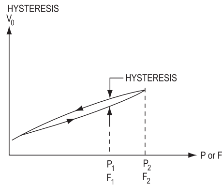
Figure 16.1.11: Hysteresis.
