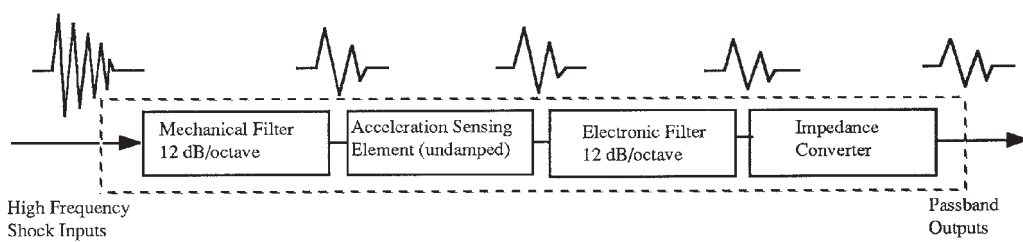
Figure 17.6.2: Integral electronic filter schematic.
