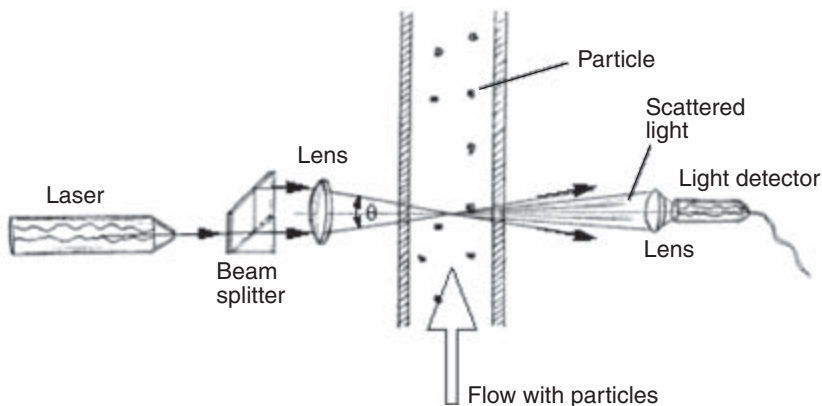
Figure 10.1.7: LDA configuration.
