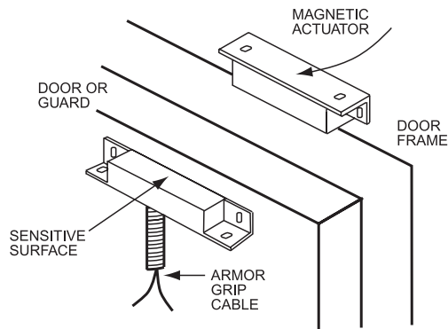
Figure 15.1.33: A proximity sensor acts as a door guard.
