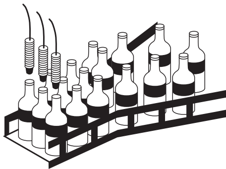
Figure 15.1.32: Proximity sensors detect bottle caps.
