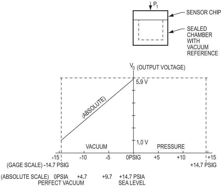
Figure 16.1.4: A signal-conditioned, absolute pressure sensor output is shown. One-volt output represents a perfect vacuum.
