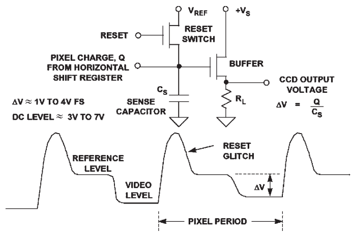
Figure 4.4.37: Output stage and waveforms.
