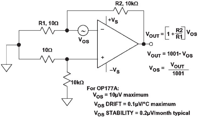
Figure 4.2.2: Measuring input offset voltage.
