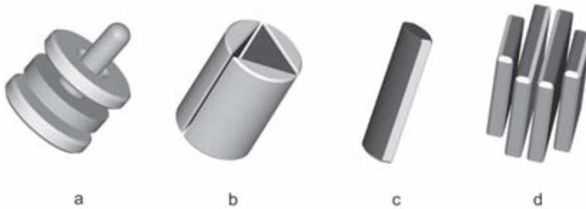
Figure 16.2.6: Different crystal element design. a) is based on longitudinal cuts. b), c) and d) are based on transverse cuts.
