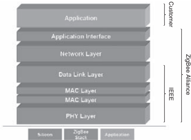
Figure 22.4.1: ZigBee stack.
