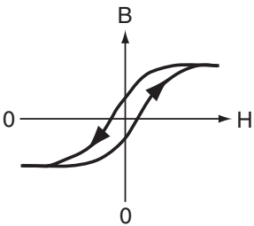
Figure 9.4.1: Hysteresis loop.
