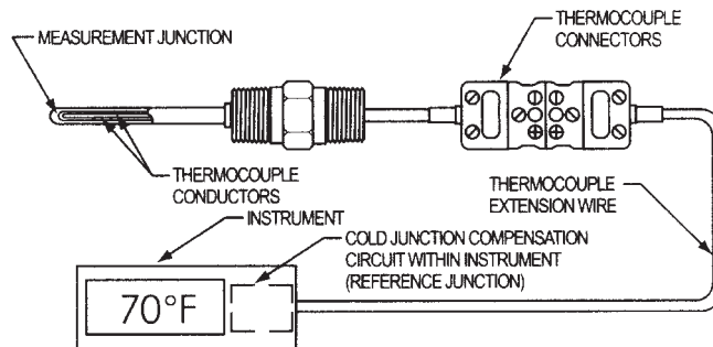
Figure 20.1.1: Thermocouple.
