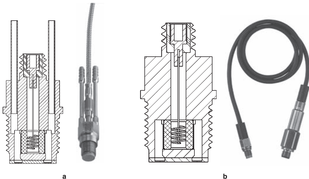
Figure 16.2.13a: Water-cooled pressure sensors M8 for engine applications.
