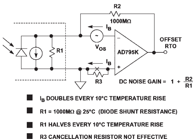
Figure 4.4.15: AD795 preamplifier DC offset errors.
