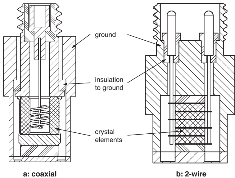
Figure 16.2.9: Ground insulated sensors. a): coaxial design. b): 2-wire design.
