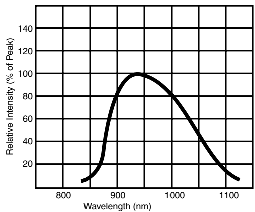
Figure 14.1.4: Typical photodiode spectral response.
