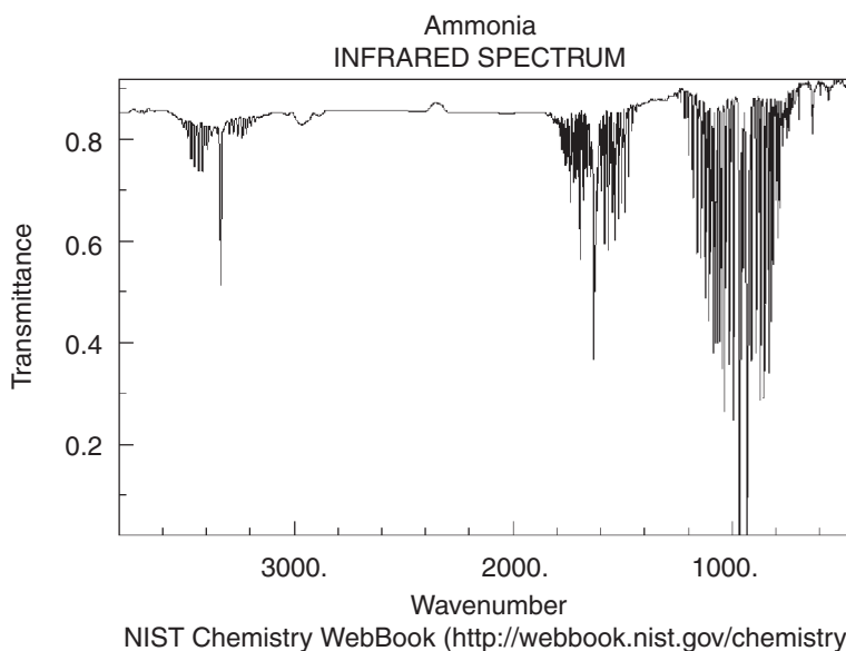
Figure 7.1.3: NH 3 spectrum.
