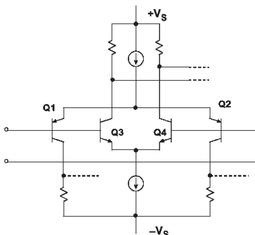
Figure 4.2.20: True rail-to-rail input stage.
