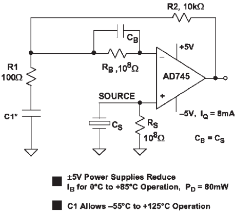
Figure 4.4.31: Gain of 100 piezoelectric sensor amplifier.
