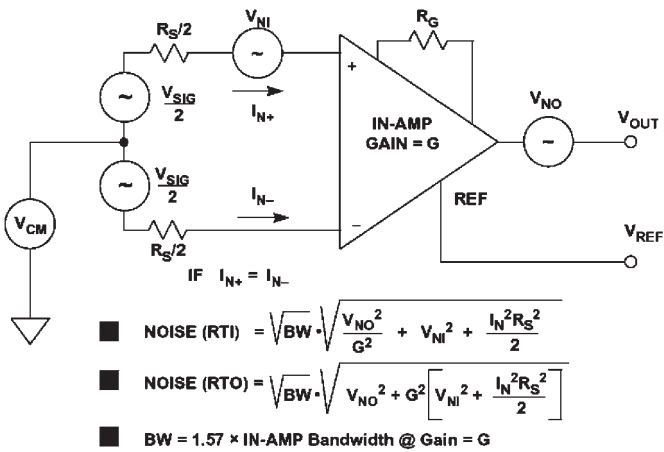
Figure 4.2.41: In-amp noise model.
