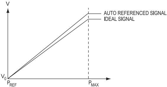
Figure 16.1.16: Auto-referenced signal.
