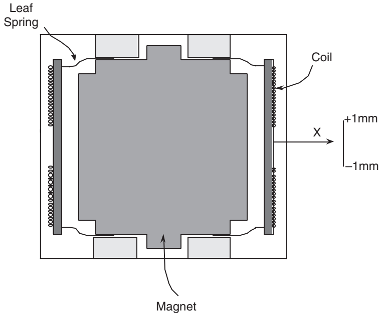
Figure 9.3.2: Geophone.
