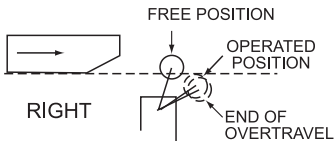
Figure 15.1.9: Operating mechanisms for limit switches should be designed so that under any operating or emergency conditions, the switch is not operated beyond its overtravel limit position. A limit switch should not be used as a mechanical stop.
