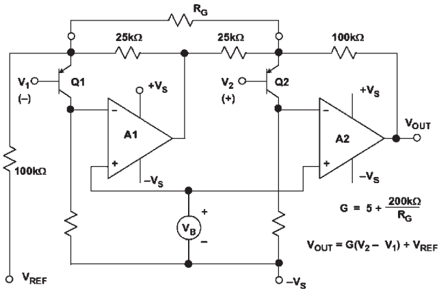
Figure 4.2.30: AD627 in-amp architecture.
