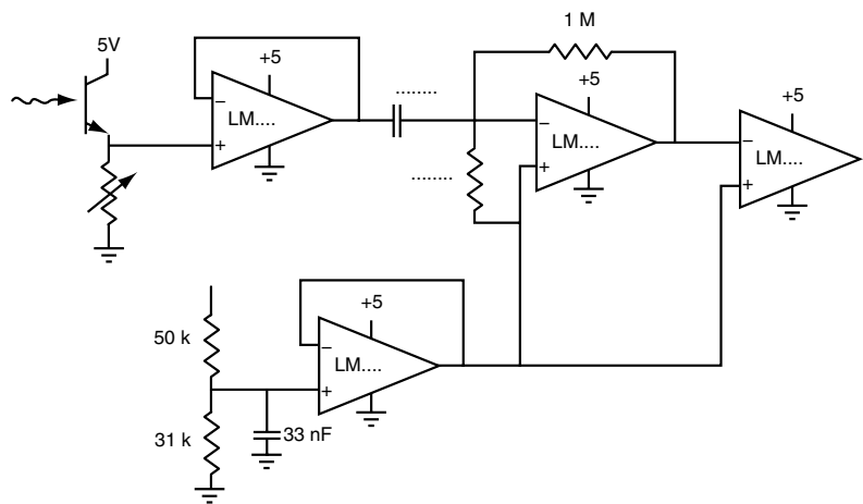
Figure 14.1.8: Phototransistor circuit.
