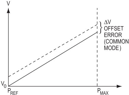
Figure 16.1.15: Common-mode errors.
