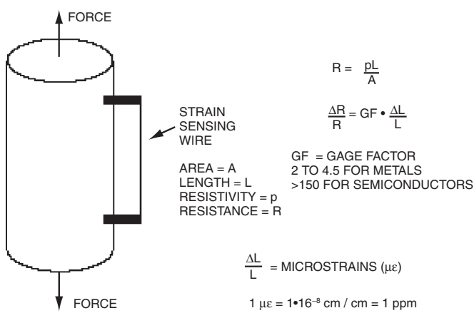
Figure 19.2.2: Unbonded wire strain gage.
