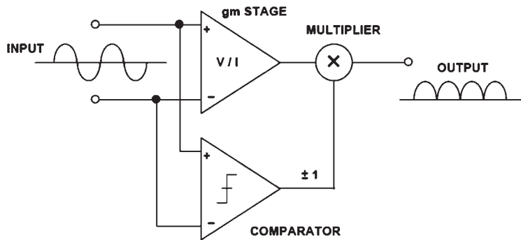
Figure 15.3.5: Precision absolute value circuit (full-wave rectifier).
