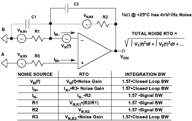
Figure 4.4.20: Amplifier noise model.
