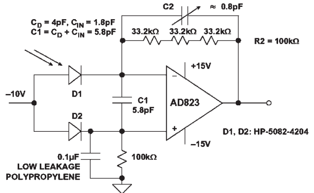
Figure 4.4.27: 2 \text{ MHz} bandwidth photodiode preamp with dark current compensation.
