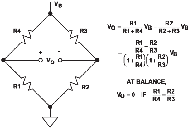
Figure 4.1.3: The Wheatstone bridge.
