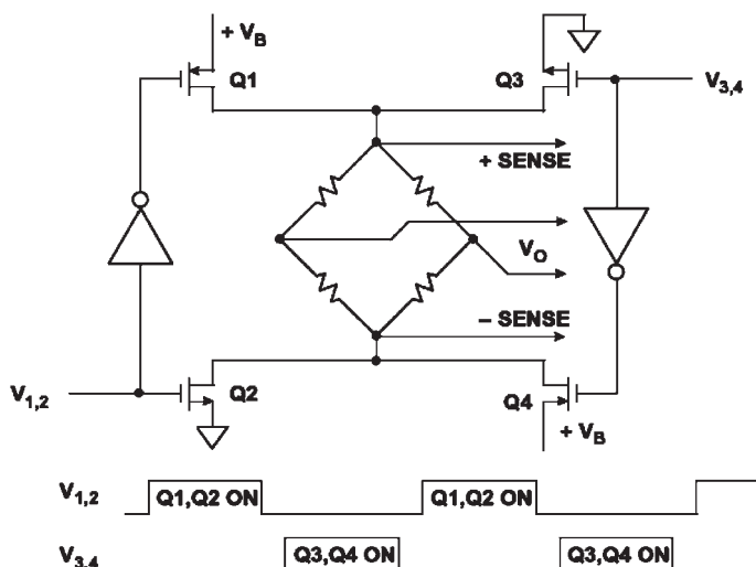
Figure 4.1.20: Simplified AC bridge drive circuit.
