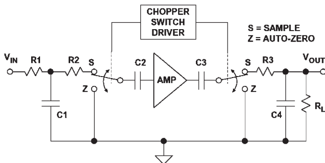
Figure 4.2.46: Classic chopper amplifier.
