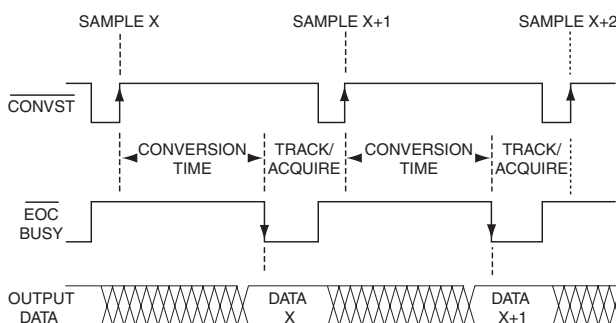
Figure 4.3.6: Typical SAR ADC timing.
