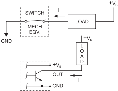
Figure 15.1.21: Typical digital Hall effect NPN output.
