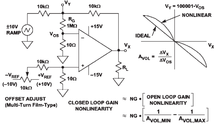
Figure 4.2.7: Circuit measures open loop gain nonlinearity.
