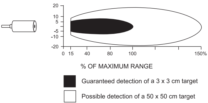
Figure 15.1.31: Target size versus beam spot.
