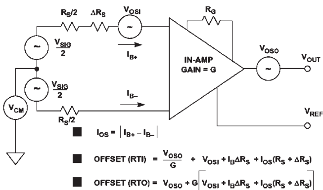
Figure 4.2.39: In-amp offset voltage model.
