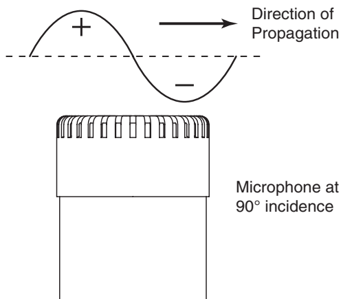
Figure 18.5.2: Wave traversing microphone diaphragm, 90^\circ incidence.
