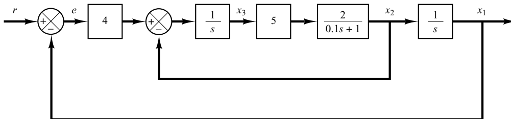
Figure 5-78 Position control system.
