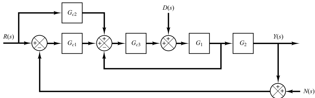
Figure 8-78 Three-degrees-of-freedom system.
